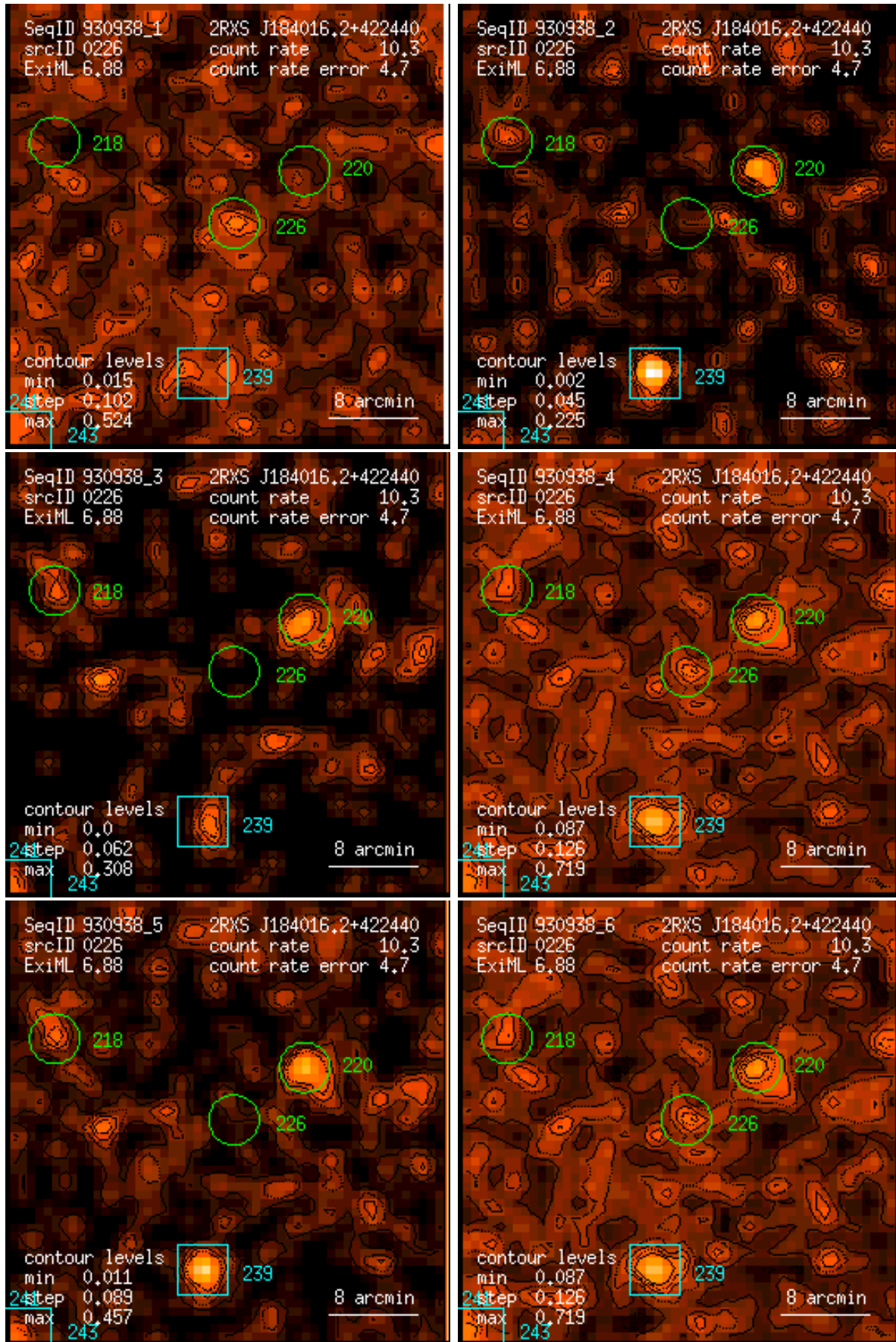
Figure 226: RASS 930938: detection 0226: band rate images, Gaussian filter: (1) PSPC channels 11 – 41, (2) 52 – 90, (3) 91 – 201, (4) 11 – 235, (5) 52 – 201, (6) 11 – 201. Broad band rates in counts/ks. Band rate contour levels in counts/ks/arcmin 2 .
