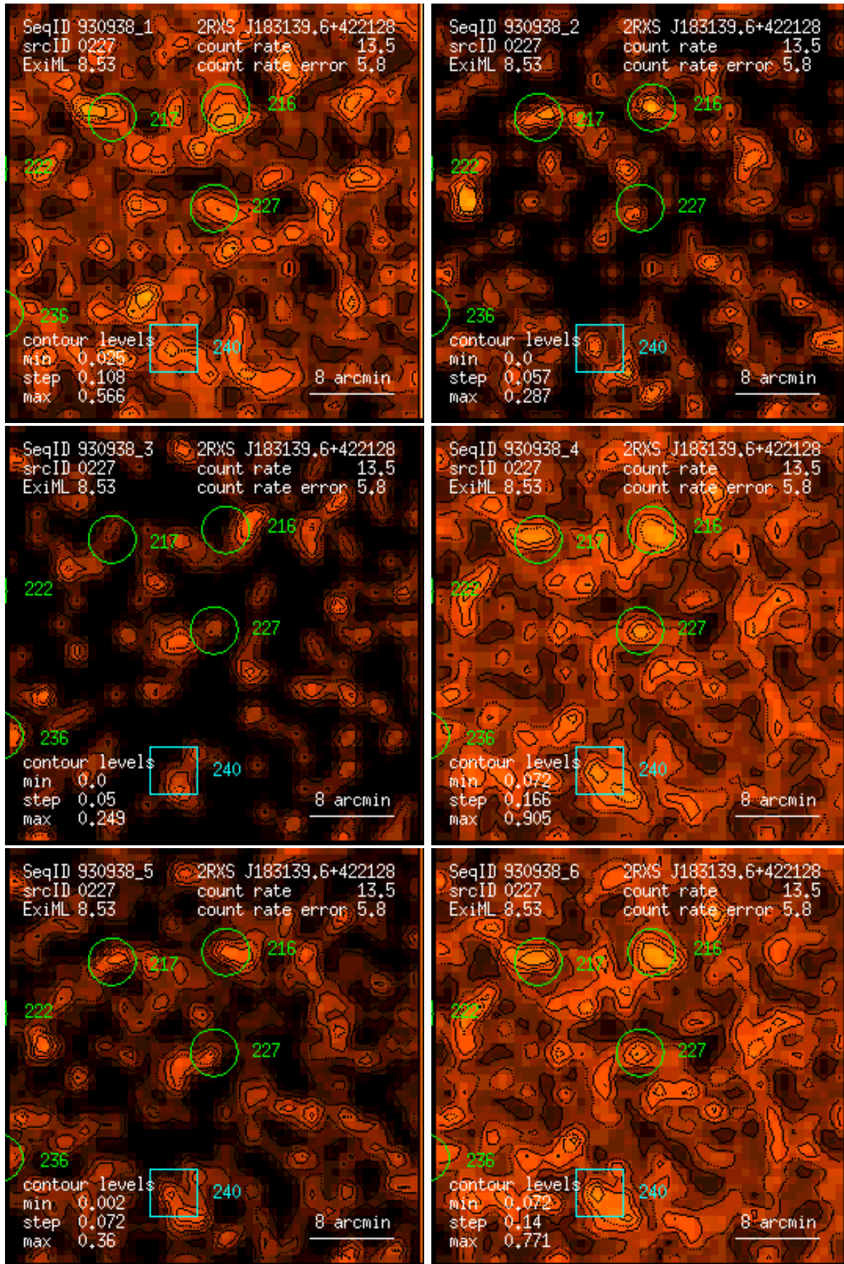
Figure 227: RASS 930938: detection 0227: band rate images, Gaussian filter: (1) PSPC channels 11 – 41, (2) 52 – 90, (3) 91 – 201, (4) 11 – 235, (5) 52 – 201, (6) 11 – 201. Broad band rates in counts/ks. Band rate contour levels in counts/ks/arcmin 2 .
