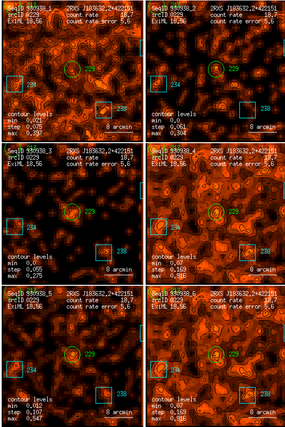
Figure 229: RASS 930938: detection 0229: band rate images, Gaussian filter: (1) PSPC channels 11 – 41, (2) 52 – 90, (3) 91 – 201, (4) 11 – 235, (5) 52 – 201, (6) 11 – 201. Broad band rates in counts/ks. Band rate contour levels in counts/ks/arcmin 2 .
