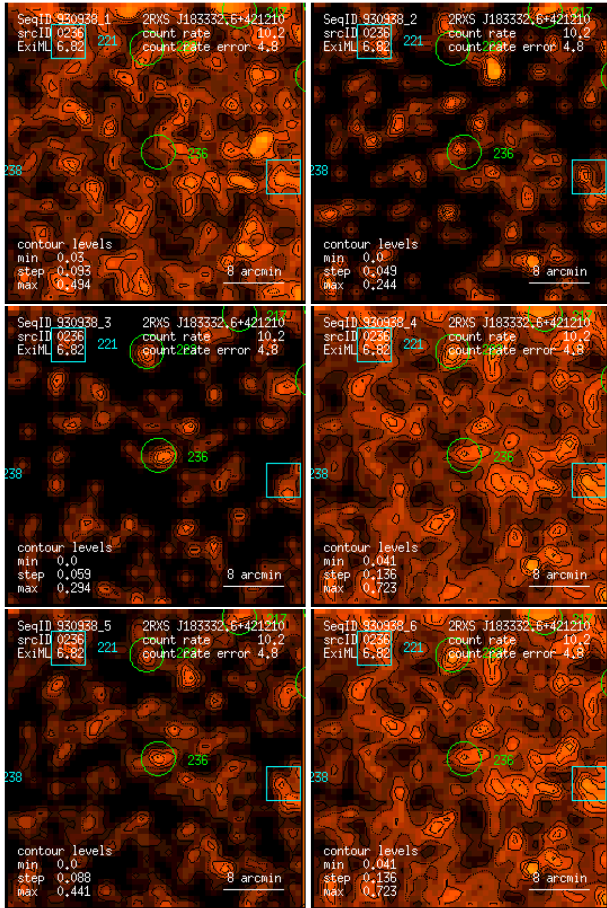
Figure 236: RASS 930938: detection 0236: band rate images, Gaussian filter: (1) PSPC channels 11 – 41, (2) 52 – 90, (3) 91 – 201, (4) 11 – 235, (5) 52 – 201, (6) 11 – 201. Broad band rates in counts/ks. Band rate contour levels in counts/ks/arcmin 2 .
