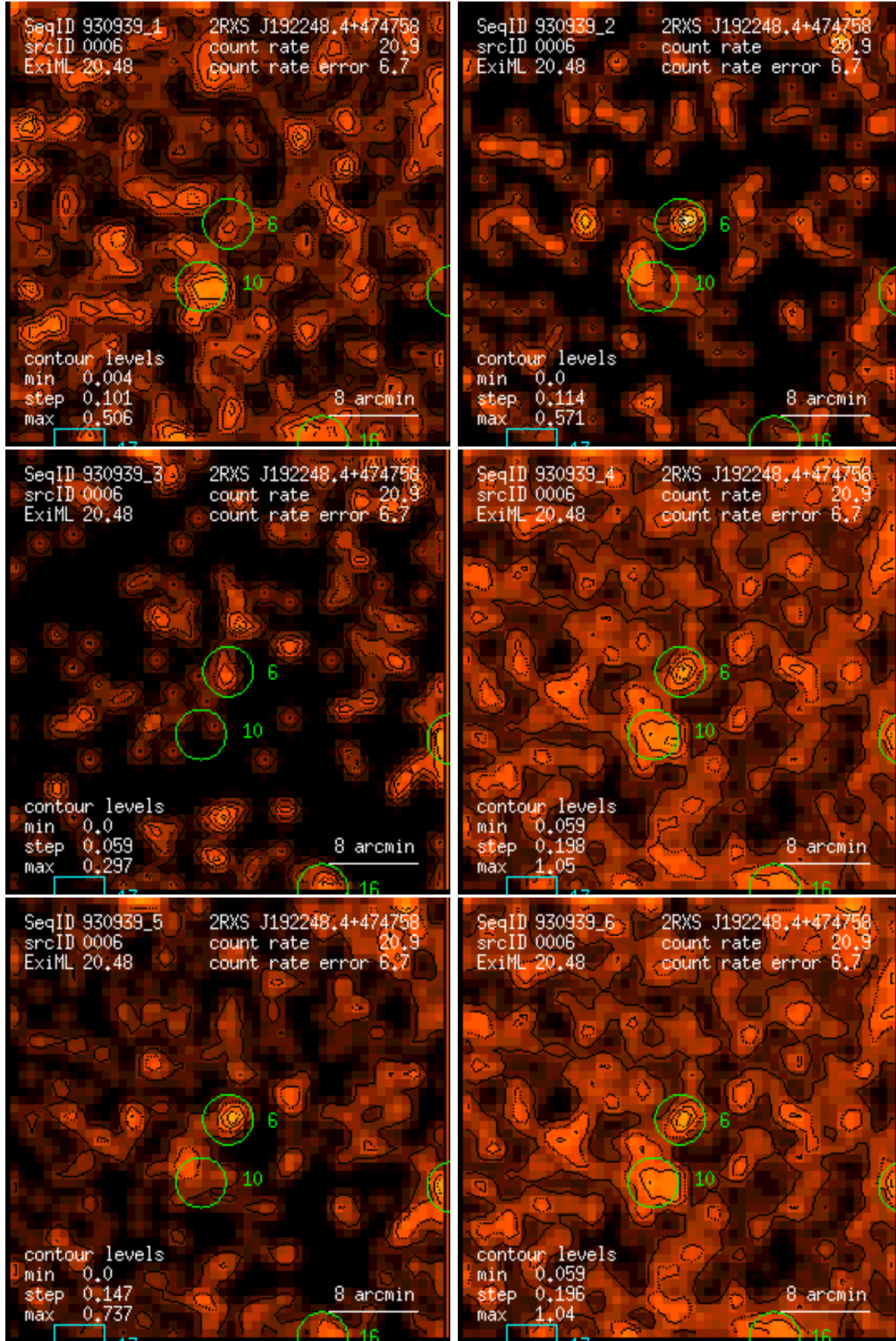
Figure 6: RASS 930939: detection 0006: band rate images, Gaussian filter: (1) PSPC channels 11 – 41, (2) 52 – 90, (3) 91 – 201, (4) 11 – 235, (5) 52 – 201, (6) 11 – 201. Broad band rates in counts/ks. Band rate contour levels in counts/ks/arcmin 2 .
