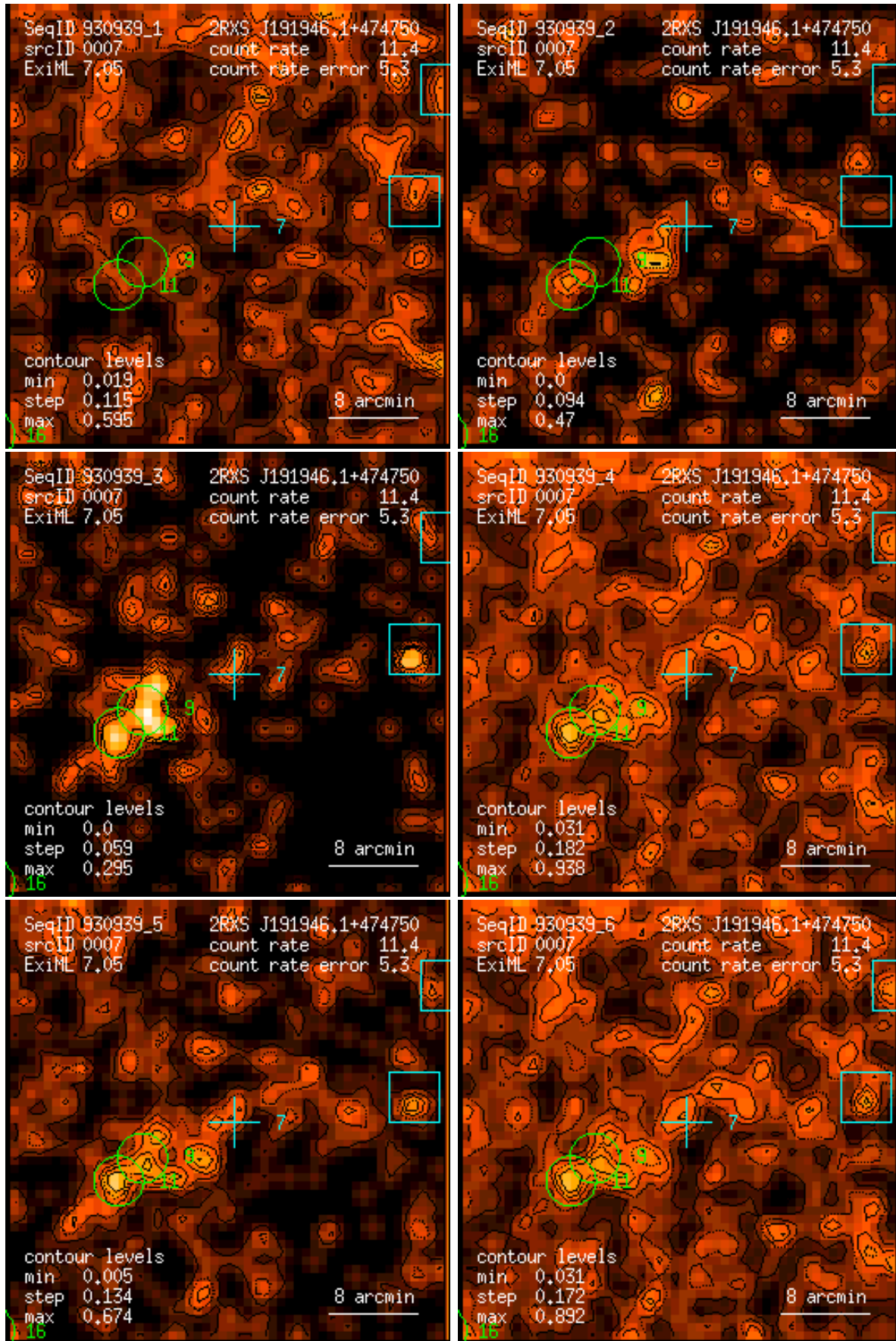
Figure 7: RASS 930939: detection 0007: band rate images, Gaussian filter: (1) PSPC channels 11 – 41, (2) 52 – 90, (3) 91 – 201, (4) 11 – 235, (5) 52 – 201, (6) 11 – 201. Broad band rates in counts/ks. Band rate contour levels in counts/ks/arcmin 2 .
