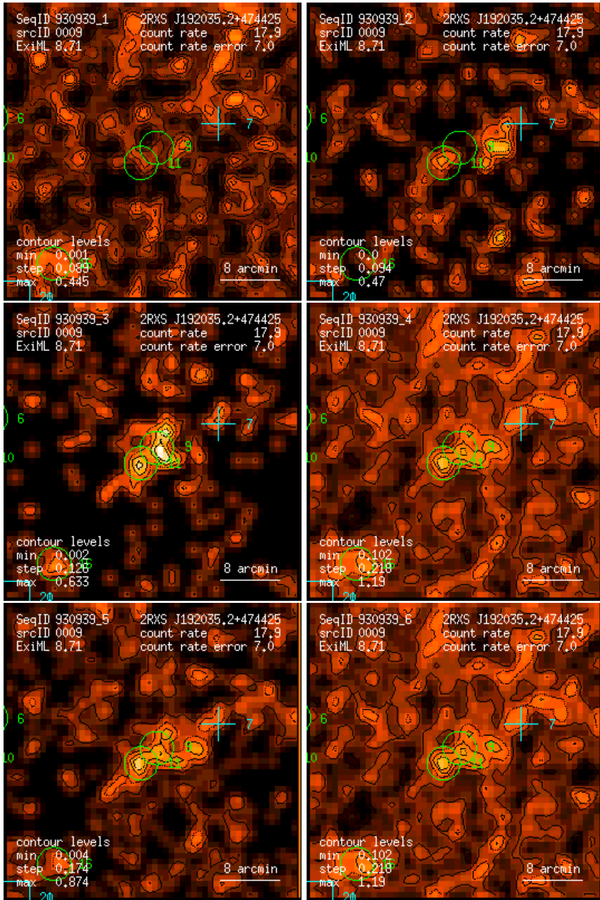
Figure 9: RASS 930939: detection 0009: band rate images, Gaussian filter: (1) PSPC channels 11 – 41, (2) 52 – 90, (3) 91 – 201, (4) 11 – 235, (5) 52 – 201, (6) 11 – 201. Broad band rates in counts/ks. Band rate contour levels in counts/ks/arcmin 2 .
