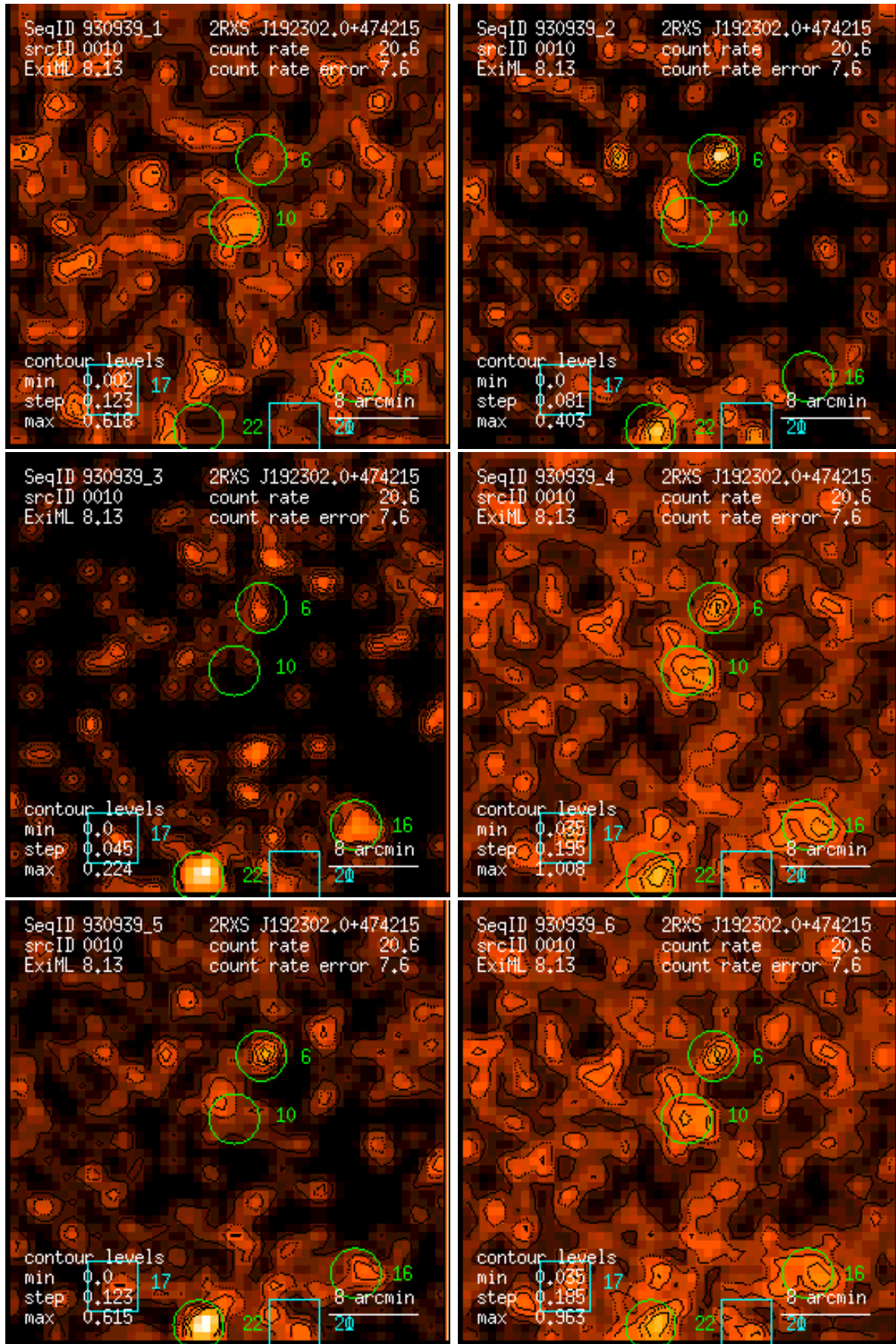
Figure 10: RASS 930939: detection 0010: band rate images, Gaussian filter: (1) PSPC channels 11 – 41, (2) 52 – 90, (3) 91 – 201, (4) 11 – 235, (5) 52 – 201, (6) 11 – 201. Broad band rates in counts/ks. Band rate contour levels in counts/ks/arcmin 2 .
