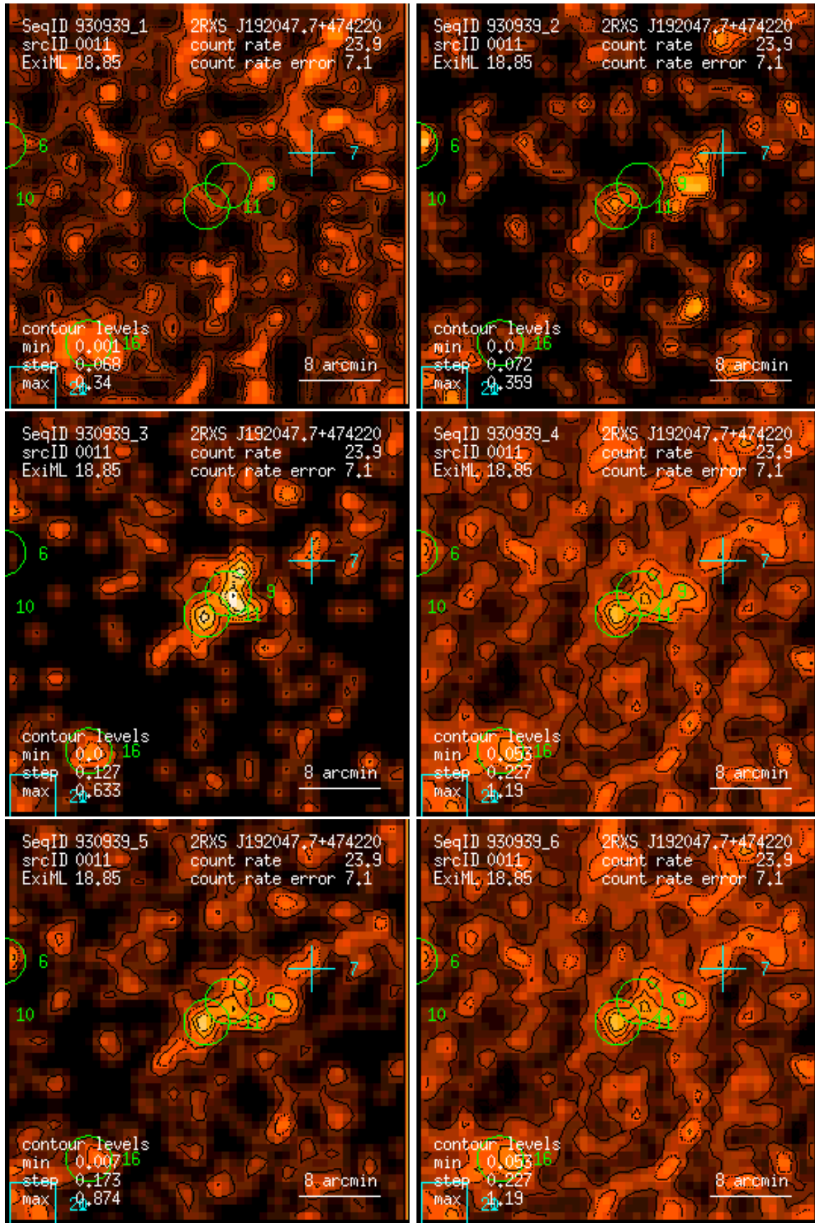
Figure 11: RASS 930939: detection 0011: band rate images, Gaussian filter: (1) PSPC channels 11 – 41, (2) 52 – 90, (3) 91 – 201, (4) 11 – 235, (5) 52 – 201, (6) 11 – 201. Broad band rates in counts/ks. Band rate contour levels in counts/ks/arcmin 2 .
