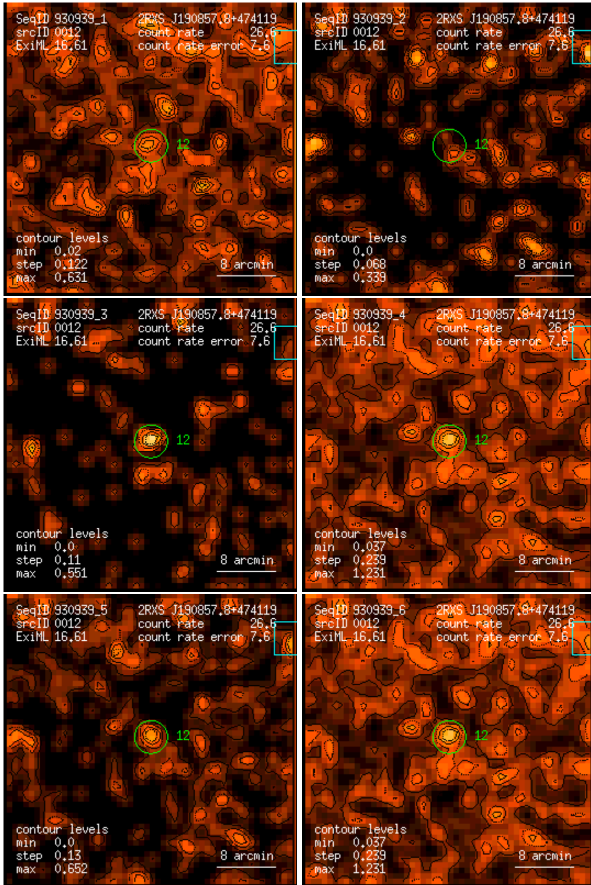
Figure 12: RASS 930939: detection 0012: band rate images, Gaussian filter: (1) PSPC channels 11 – 41, (2) 52 – 90, (3) 91 – 201, (4) 11 – 235, (5) 52 – 201, (6) 11 – 201. Broad band rates in counts/ks. Band rate contour levels in counts/ks/arcmin 2 .
