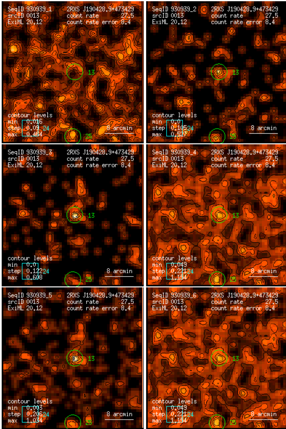
Figure 13: RASS 930939: detection 0013: band rate images, Gaussian filter: (1) PSPC channels 11 – 41, (2) 52 – 90, (3) 91 – 201, (4) 11 – 235, (5) 52 – 201, (6) 11 – 201. Broad band rates in counts/ks. Band rate contour levels in counts/ks/arcmin 2 .
