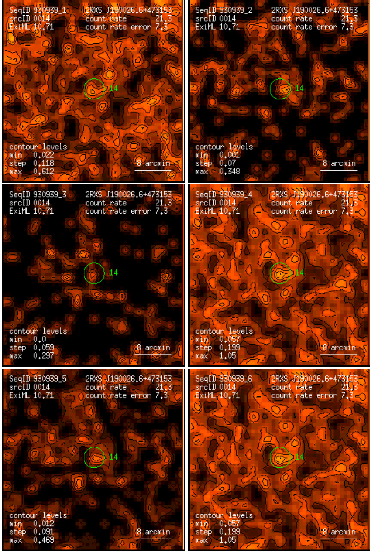
Figure 14: RASS 930939: detection 0014: band rate images, Gaussian filter: (1) PSPC channels 11 – 41, (2) 52 – 90, (3) 91 – 201, (4) 11 – 235, (5) 52 – 201, (6) 11 – 201. Broad band rates in counts/ks. Band rate contour levels in counts/ks/arcmin 2 .
