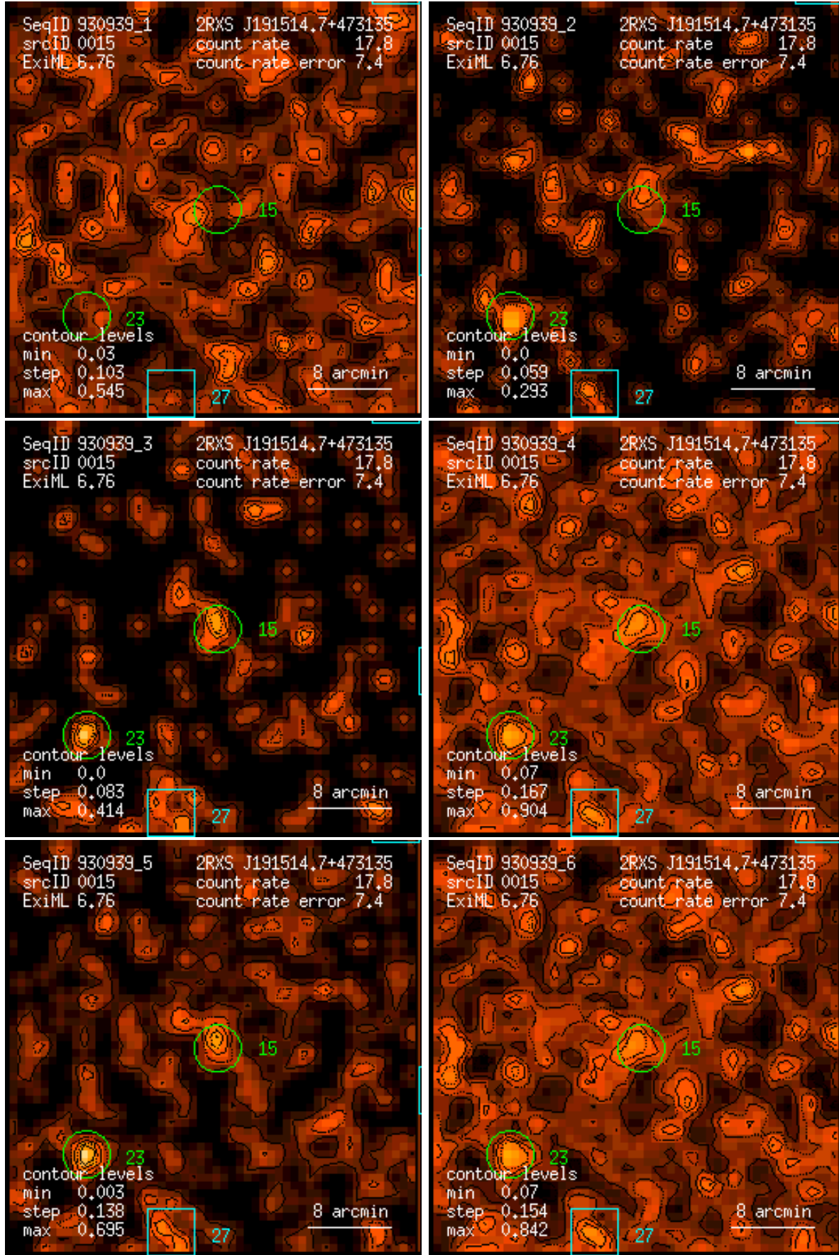
Figure 15: RASS 930939: detection 0015: band rate images, Gaussian filter: (1) PSPC channels 11 – 41, (2) 52 – 90, (3) 91 – 201, (4) 11 – 235, (5) 52 – 201, (6) 11 – 201. Broad band rates in counts/ks. Band rate contour levels in counts/ks/arcmin 2 .
