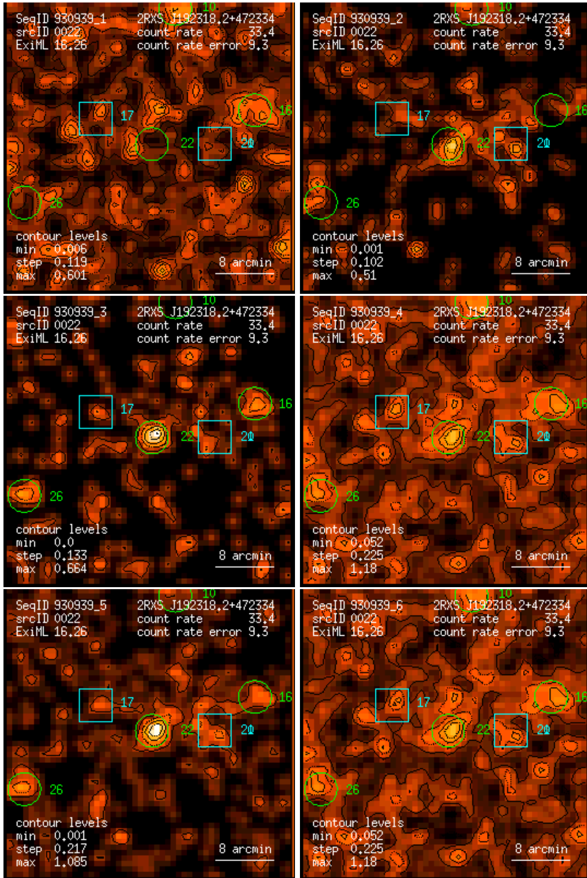
Figure 22: RASS 930939: detection 0022: band rate images, Gaussian filter: (1) PSPC channels 11 – 41, (2) 52 – 90, (3) 91 – 201, (4) 11 – 235, (5) 52 – 201, (6) 11 – 201. Broad band rates in counts/ks. Band rate contour levels in counts/ks/arcmin 2 .
