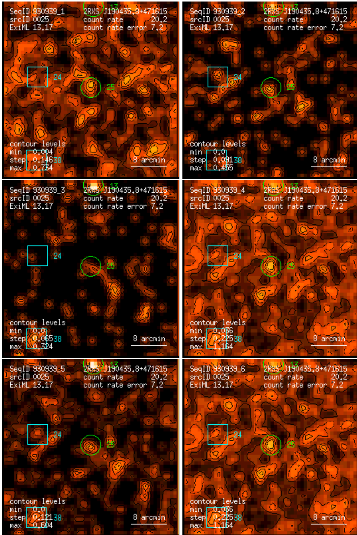
Figure 25: RASS 930939: detection 0025: band rate images, Gaussian filter: (1) PSPC channels 11 – 41, (2) 52 – 90, (3) 91 – 201, (4) 11 – 235, (5) 52 – 201, (6) 11 – 201. Broad band rates in counts/ks. Band rate contour levels in counts/ks/arcmin 2 .
