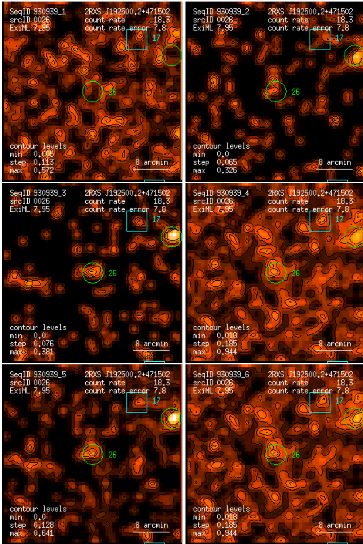
Figure 26: RASS 930939: detection 0026: band rate images, Gaussian filter: (1) PSPC channels 11 – 41, (2) 52 – 90, (3) 91 – 201, (4) 11 – 235, (5) 52 – 201, (6) 11 – 201. Broad band rates in counts/ks. Band rate contour levels in counts/ks/arcmin 2 .
