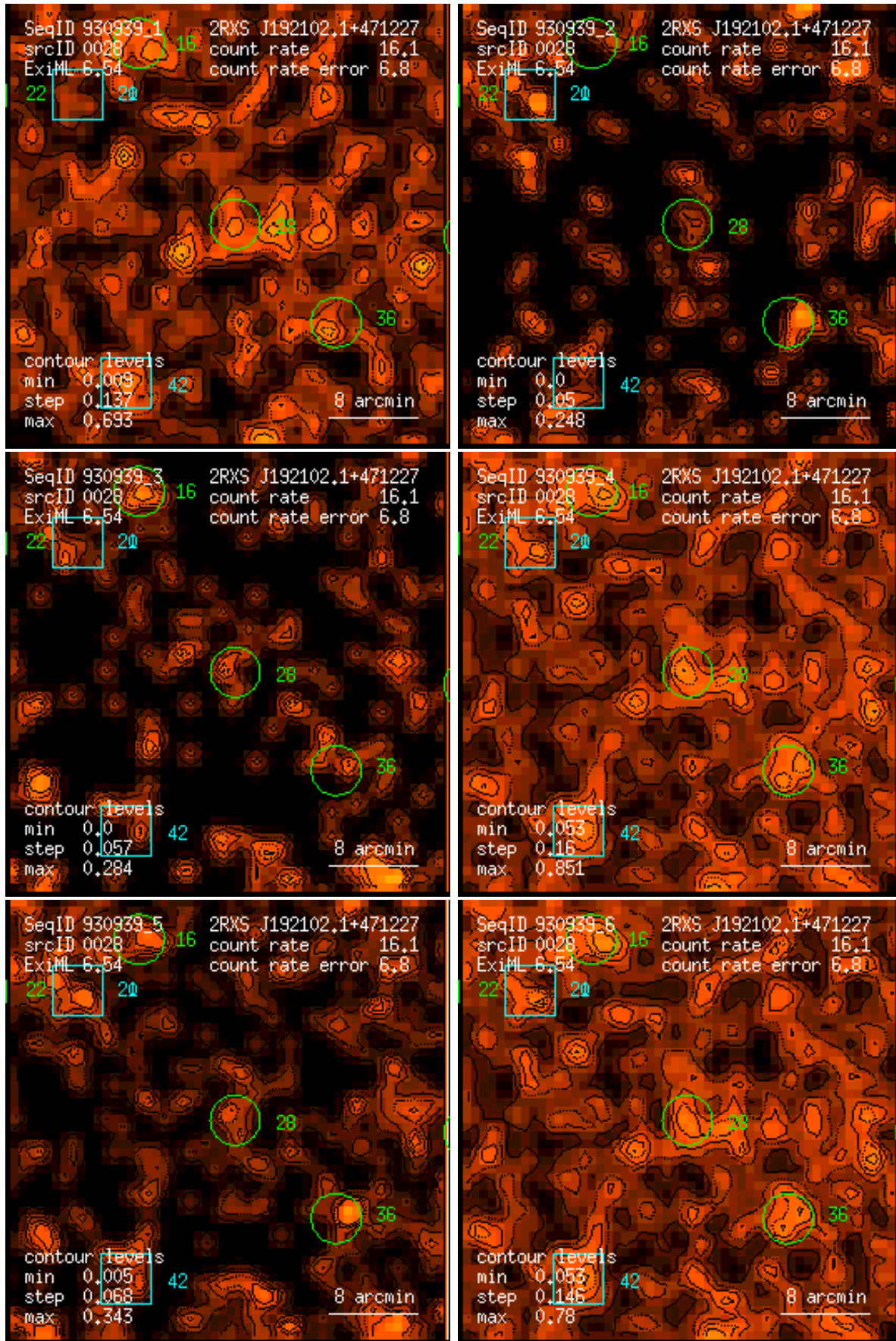
Figure 28: RASS 930939: detection 0028: band rate images, Gaussian filter: (1) PSPC channels 11 – 41, (2) 52 – 90, (3) 91 – 201, (4) 11 – 235, (5) 52 – 201, (6) 11 – 201. Broad band rates in counts/ks. Band rate contour levels in counts/ks/arcmin 2 .
