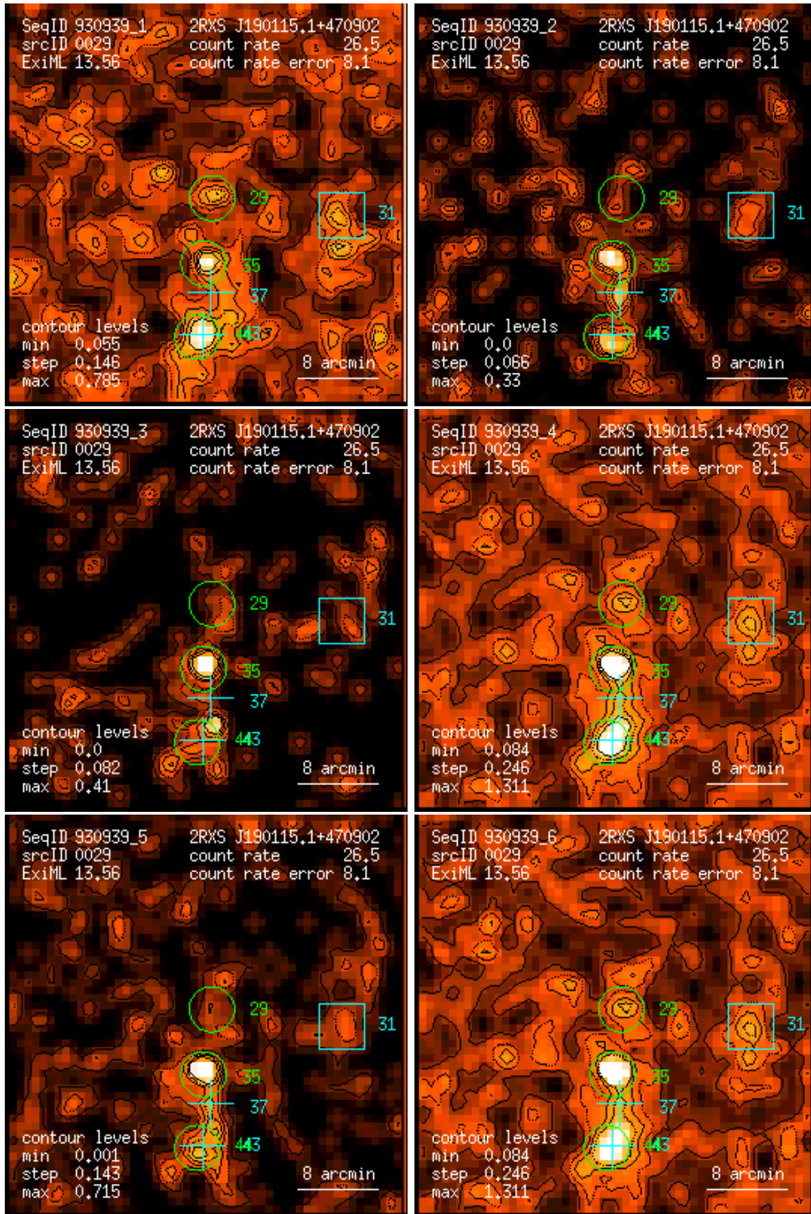
Figure 29: RASS 930939: detection 0029: band rate images, Gaussian filter: (1) PSPC channels 11 – 41, (2) 52 – 90, (3) 91 – 201, (4) 11 – 235, (5) 52 – 201, (6) 11 – 201. Broad band rates in counts/ks. Band rate contour levels in counts/ks/arcmin 2 .
