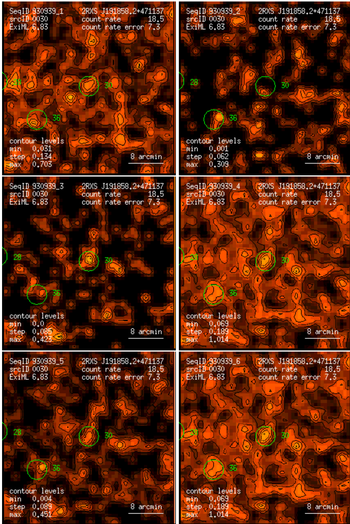
Figure 30: RASS 930939: detection 0030: band rate images, Gaussian filter: (1) PSPC channels 11 – 41, (2) 52 – 90, (3) 91 – 201, (4) 11 – 235, (5) 52 – 201, (6) 11 – 201. Broad band rates in counts/ks. Band rate contour levels in counts/ks/arcmin 2 .
