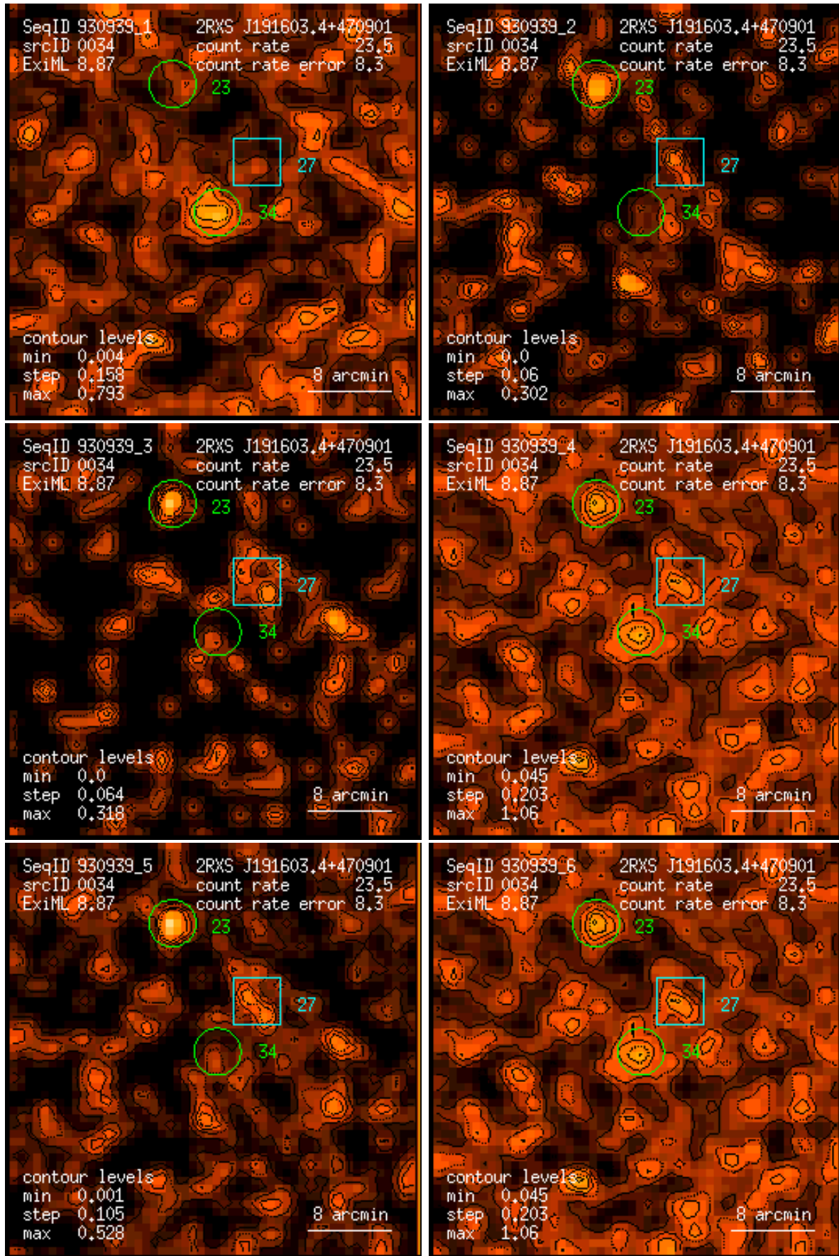
Figure 34: RASS 930939: detection 0034: band rate images, Gaussian filter: (1) PSPC channels 11 – 41, (2) 52 – 90, (3) 91 – 201, (4) 11 – 235, (5) 52 – 201, (6) 11 – 201. Broad band rates in counts/ks. Band rate contour levels in counts/ks/arcmin 2 .
