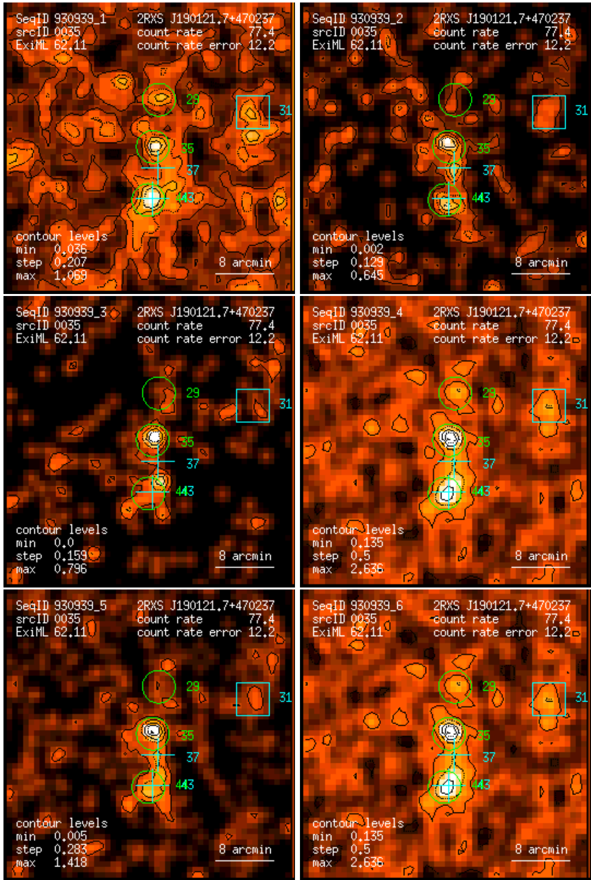
Figure 35: RASS 930939: detection 0035: band rate images, Gaussian filter: (1) PSPC channels 11 – 41, (2) 52 – 90, (3) 91 – 201, (4) 11 – 235, (5) 52 – 201, (6) 11 – 201. Broad band rates in counts/ks. Band rate contour levels in counts/ks/arcmin 2 .
