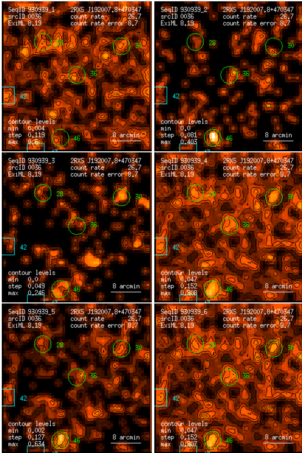
Figure 36: RASS 930939: detection 0036: band rate images, Gaussian filter: (1) PSPC channels 11 – 41, (2) 52 – 90, (3) 91 – 201, (4) 11 – 235, (5) 52 – 201, (6) 11 – 201. Broad band rates in counts/ks. Band rate contour levels in counts/ks/arcmin 2 .
