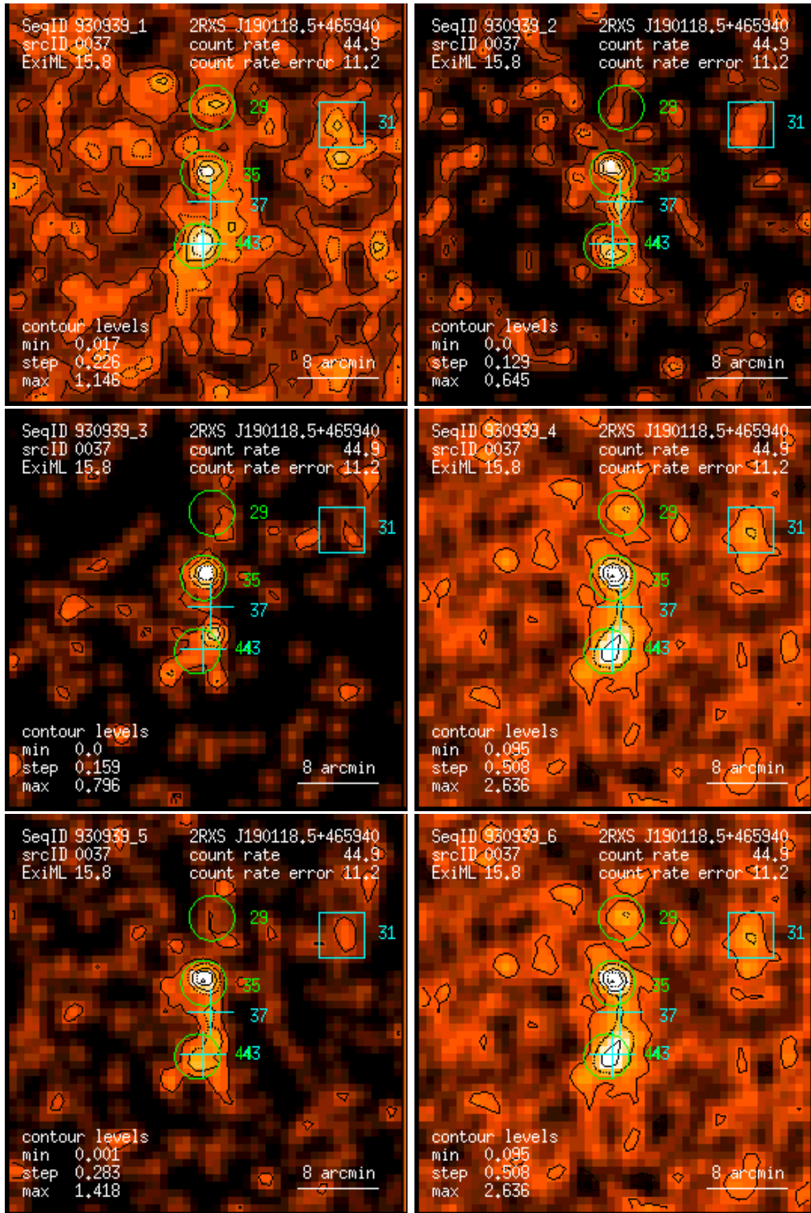
Figure 37: RASS 930939: detection 0037: band rate images, Gaussian filter: (1) PSPC channels 11 – 41, (2) 52 – 90, (3) 91 – 201, (4) 11 – 235, (5) 52 – 201, (6) 11 – 201. Broad band rates in counts/ks. Band rate contour levels in counts/ks/arcmin 2 .
