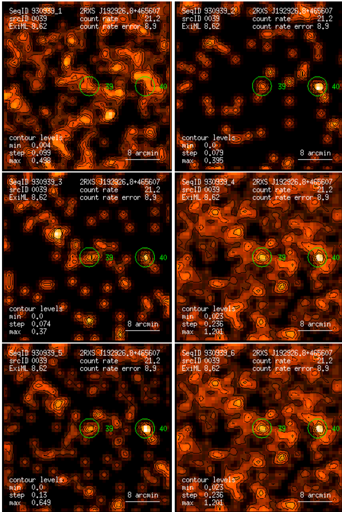
Figure 39: RASS 930939: detection 0039: band rate images, Gaussian filter: (1) PSPC channels 11 – 41, (2) 52 – 90, (3) 91 – 201, (4) 11 – 235, (5) 52 – 201, (6) 11 – 201. Broad band rates in counts/ks. Band rate contour levels in counts/ks/arcmin 2 .
