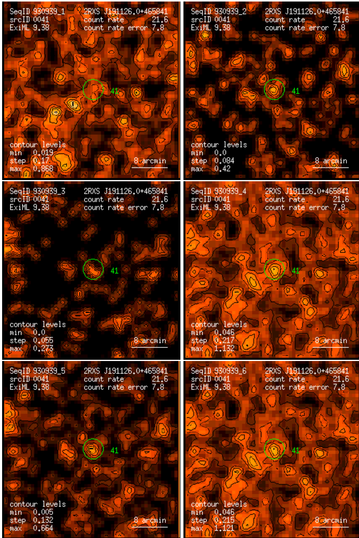
Figure 41: RASS 930939: detection 0041: band rate images, Gaussian filter: (1) PSPC channels 11 – 41, (2) 52 – 90, (3) 91 – 201, (4) 11 – 235, (5) 52 – 201, (6) 11 – 201. Broad band rates in counts/ks. Band rate contour levels in counts/ks/arcmin 2 .
