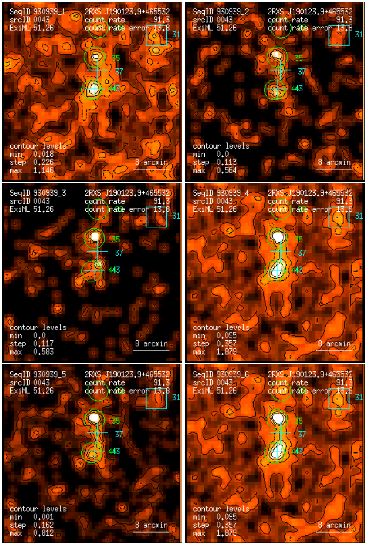
Figure 43: RASS 930939: detection 0043: band rate images, Gaussian filter: (1) PSPC channels 11 – 41, (2) 52 – 90, (3) 91 – 201, (4) 11 – 235, (5) 52 – 201, (6) 11 – 201. Broad band rates in counts/ks. Band rate contour levels in counts/ks/arcmin 2 .
