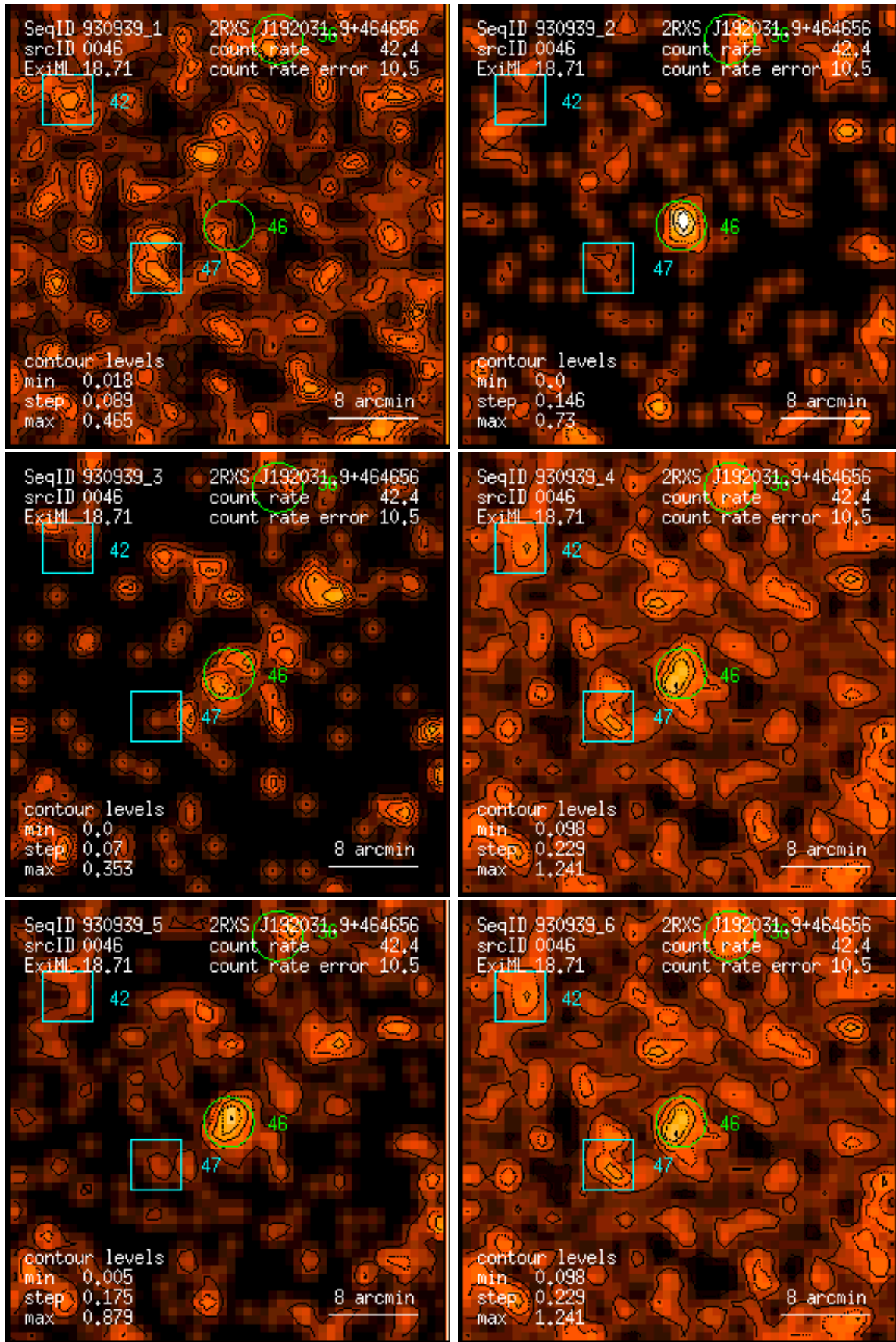
Figure 46: RASS 930939: detection 0046: band rate images, Gaussian filter: (1) PSPC channels 11 – 41, (2) 52 – 90, (3) 91 – 201, (4) 11 – 235, (5) 52 – 201, (6) 11 – 201. Broad band rates in counts/ks. Band rate contour levels in counts/ks/arcmin 2 .
