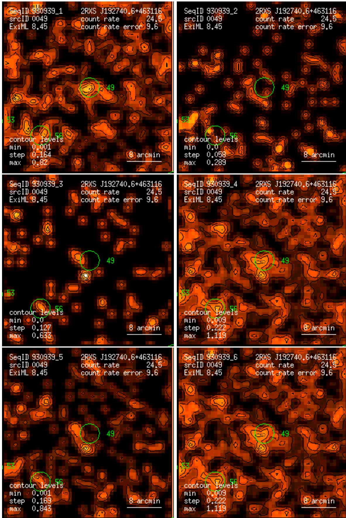
Figure 49: RASS 930939: detection 0049: band rate images, Gaussian filter: (1) PSPC channels 11 – 41, (2) 52 – 90, (3) 91 – 201, (4) 11 – 235, (5) 52 – 201, (6) 11 – 201. Broad band rates in counts/ks. Band rate contour levels in counts/ks/arcmin 2 .
