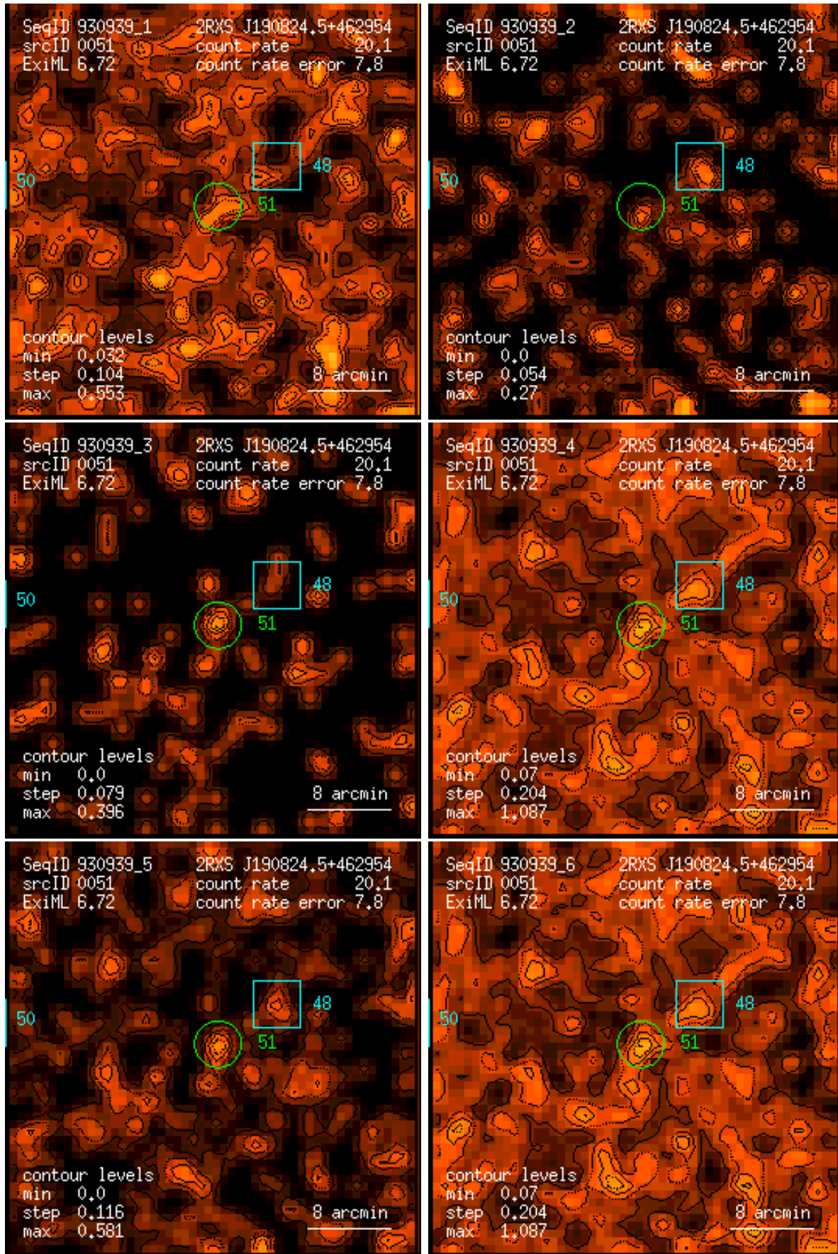
Figure 51: RASS 930939: detection 0051: band rate images, Gaussian filter: (1) PSPC channels 11 – 41, (2) 52 – 90, (3) 91 – 201, (4) 11 – 235, (5) 52 – 201, (6) 11 – 201. Broad band rates in counts/ks. Band rate contour levels in counts/ks/arcmin 2 .
