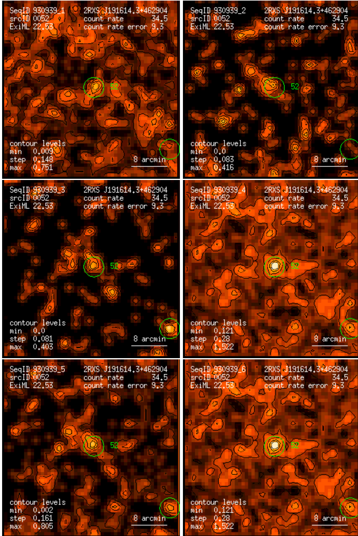
Figure 52: RASS 930939: detection 0052: band rate images, Gaussian filter: (1) PSPC channels 11 – 41, (2) 52 – 90, (3) 91 – 201, (4) 11 – 235, (5) 52 – 201, (6) 11 – 201. Broad band rates in counts/ks. Band rate contour levels in counts/ks/arcmin 2 .
