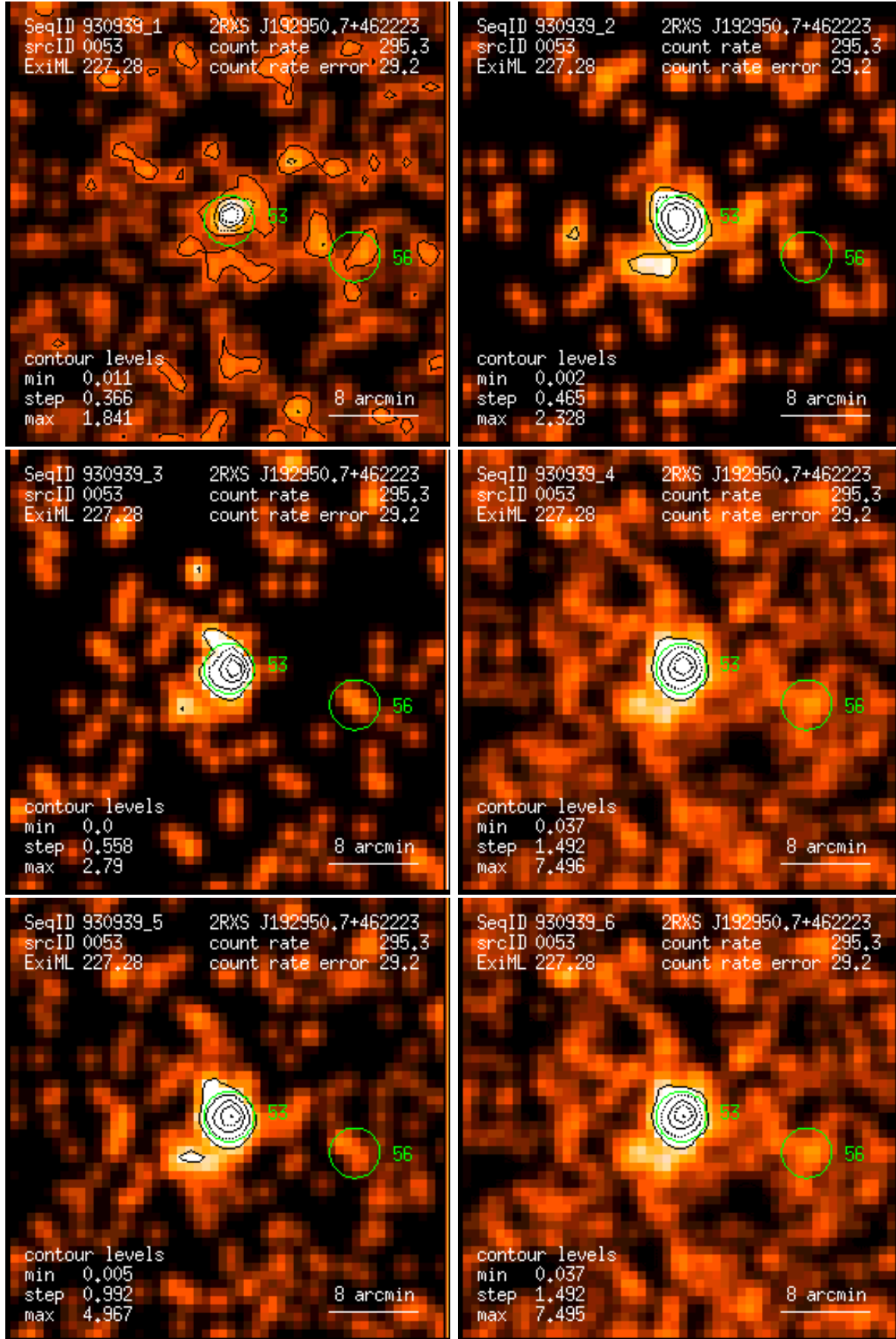
Figure 53: RASS 930939: detection 0053: band rate images, Gaussian filter: (1) PSPC channels 11 – 41, (2) 52 – 90, (3) 91 – 201, (4) 11 – 235, (5) 52 – 201, (6) 11 – 201. Broad band rates in counts/ks. Band rate contour levels in counts/ks/arcmin 2 .
