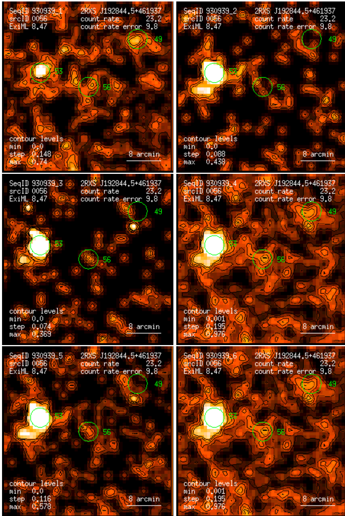
Figure 56: RASS 930939: detection 0056: band rate images, Gaussian filter: (1) PSPC channels 11 – 41, (2) 52 – 90, (3) 91 – 201, (4) 11 – 235, (5) 52 – 201, (6) 11 – 201. Broad band rates in counts/ks. Band rate contour levels in counts/ks/arcmin 2 .
