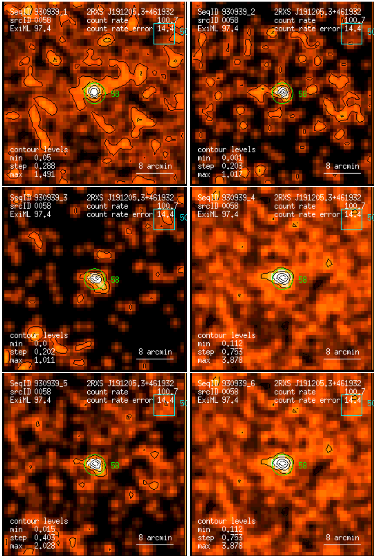
Figure 58: RASS 930939: detection 0058: band rate images, Gaussian filter: (1) PSPC channels 11 – 41, (2) 52 – 90, (3) 91 – 201, (4) 11 – 235, (5) 52 – 201, (6) 11 – 201. Broad band rates in counts/ks. Band rate contour levels in counts/ks/arcmin 2 .
