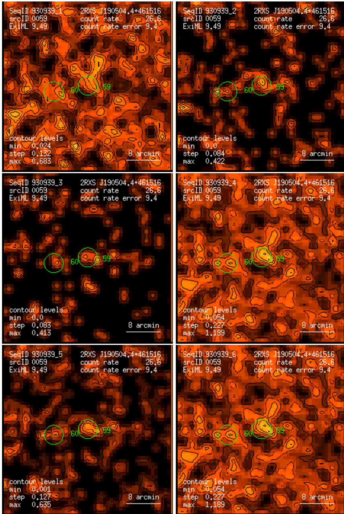
Figure 59: RASS 930939: detection 0059: band rate images, Gaussian filter: (1) PSPC channels 11 – 41, (2) 52 – 90, (3) 91 – 201, (4) 11 – 235, (5) 52 – 201, (6) 11 – 201. Broad band rates in counts/ks. Band rate contour levels in counts/ks/arcmin 2 .
