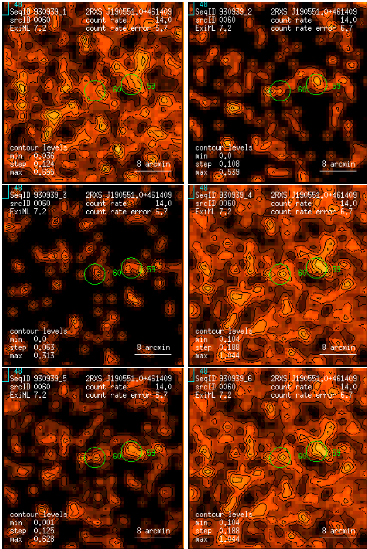
Figure 60: RASS 930939: detection 0060: band rate images, Gaussian filter: (1) PSPC channels 11 – 41, (2) 52 – 90, (3) 91 – 201, (4) 11 – 235, (5) 52 – 201, (6) 11 – 201. Broad band rates in counts/ks. Band rate contour levels in counts/ks/arcmin 2 .
