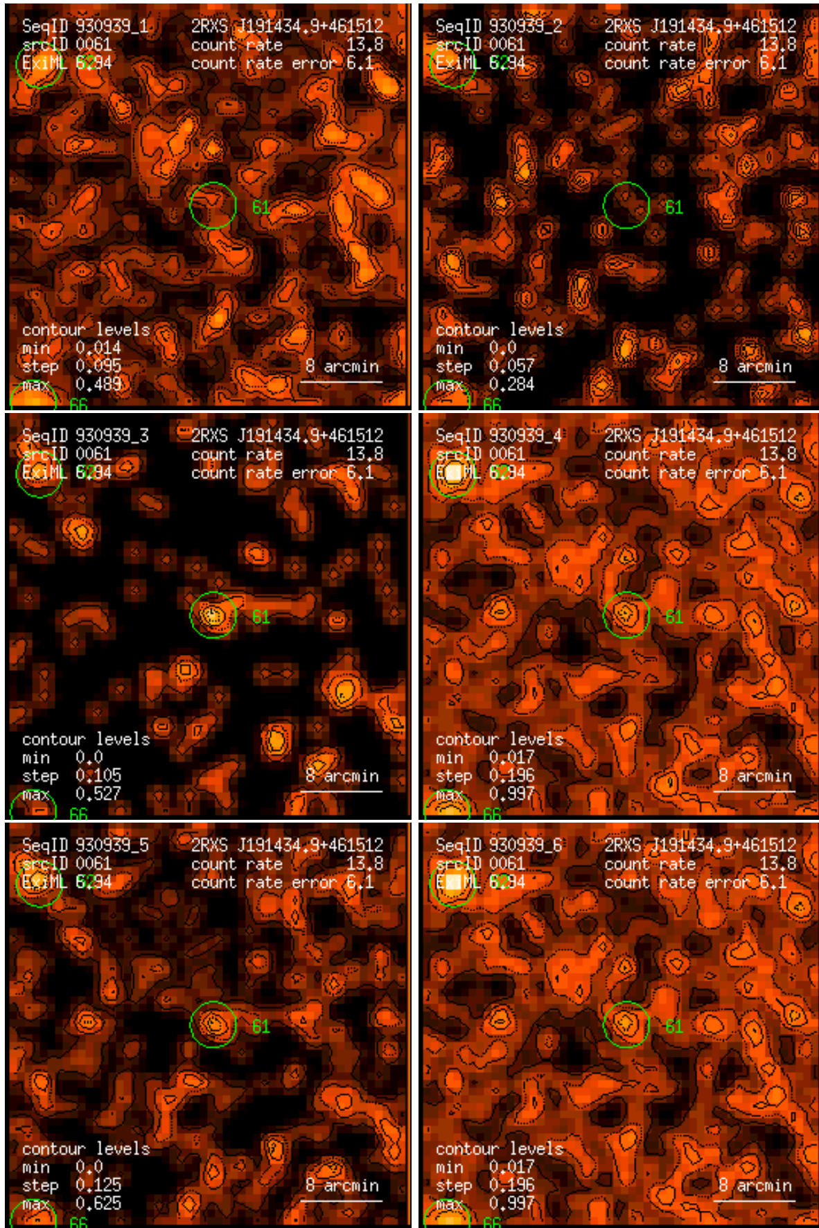
Figure 61: RASS 930939: detection 0061: band rate images, Gaussian filter: (1) PSPC channels 11 – 41, (2) 52 – 90, (3) 91 – 201, (4) 11 – 235, (5) 52 – 201, (6) 11 – 201. Broad band rates in counts/ks. Band rate contour levels in counts/ks/arcmin 2 .
