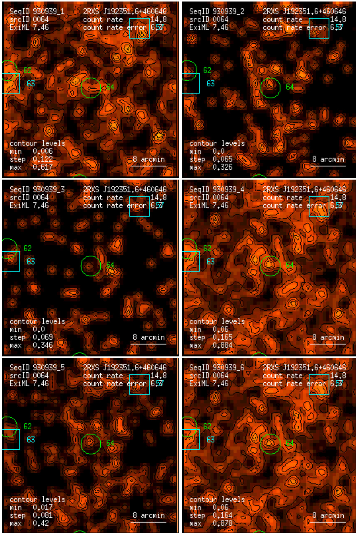
Figure 64: RASS 930939: detection 0064: band rate images, Gaussian filter: (1) PSPC channels 11 – 41, (2) 52 – 90, (3) 91 – 201, (4) 11 – 235, (5) 52 – 201, (6) 11 – 201. Broad band rates in counts/ks. Band rate contour levels in counts/ks/arcmin 2 .
