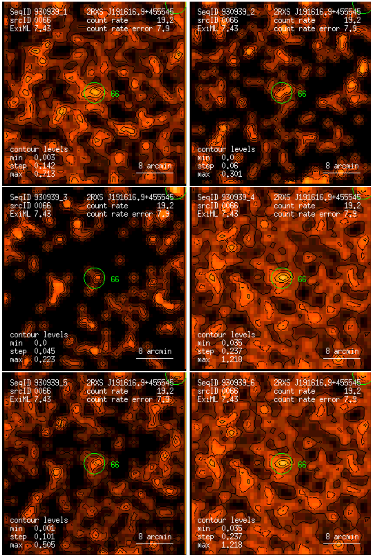
Figure 66: RASS 930939: detection 0066: band rate images, Gaussian filter: (1) PSPC channels 11 – 41, (2) 52 – 90, (3) 91 – 201, (4) 11 – 235, (5) 52 – 201, (6) 11 – 201. Broad band rates in counts/ks. Band rate contour levels in counts/ks/arcmin 2 .
