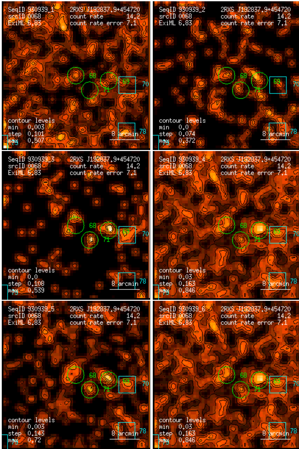
Figure 68: RASS 930939: detection 0068: band rate images, Gaussian filter: (1) PSPC channels 11 – 41, (2) 52 – 90, (3) 91 – 201, (4) 11 – 235, (5) 52 – 201, (6) 11 – 201. Broad band rates in counts/ks. Band rate contour levels in counts/ks/arcmin 2 .
