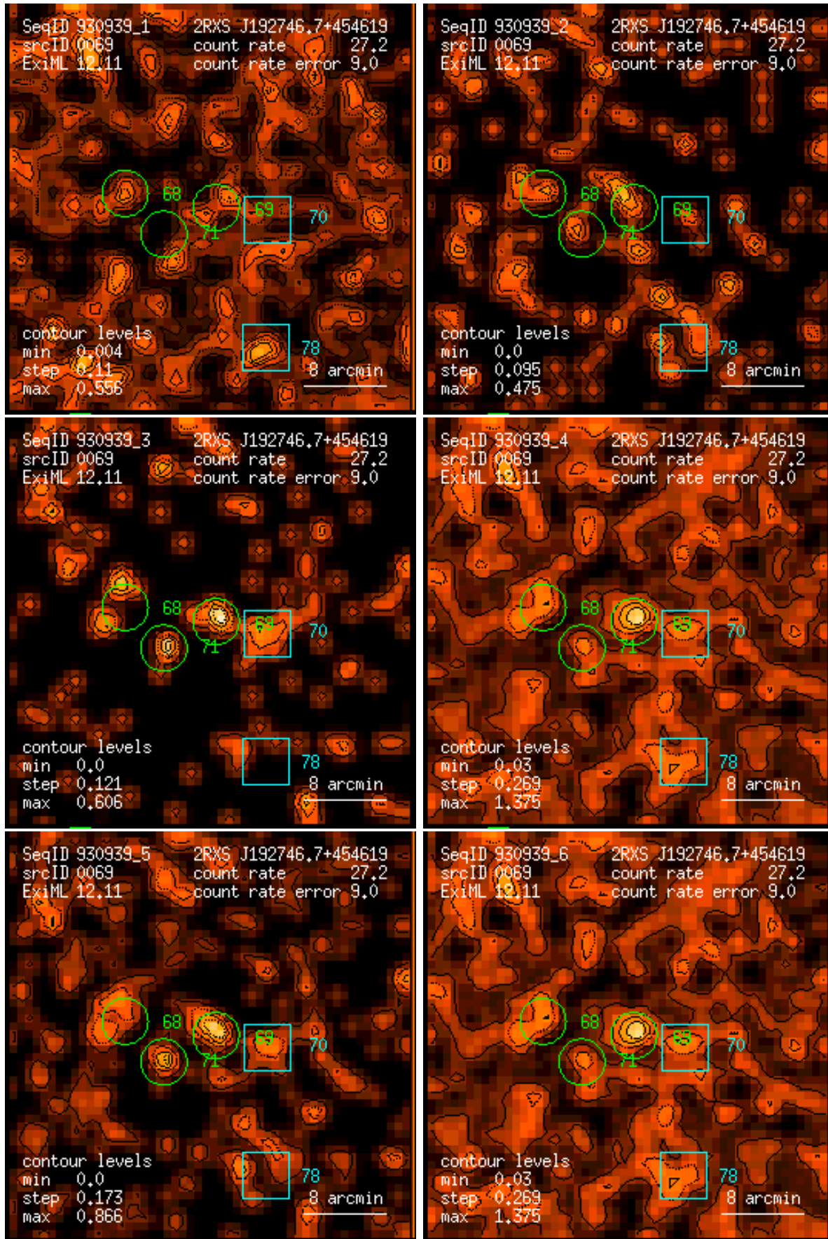
Figure 69: RASS 930939: detection 0069: band rate images, Gaussian filter: (1) PSPC channels 11 – 41, (2) 52 – 90, (3) 91 – 201, (4) 11 – 235, (5) 52 – 201, (6) 11 – 201. Broad band rates in counts/ks. Band rate contour levels in counts/ks/arcmin 2 .
