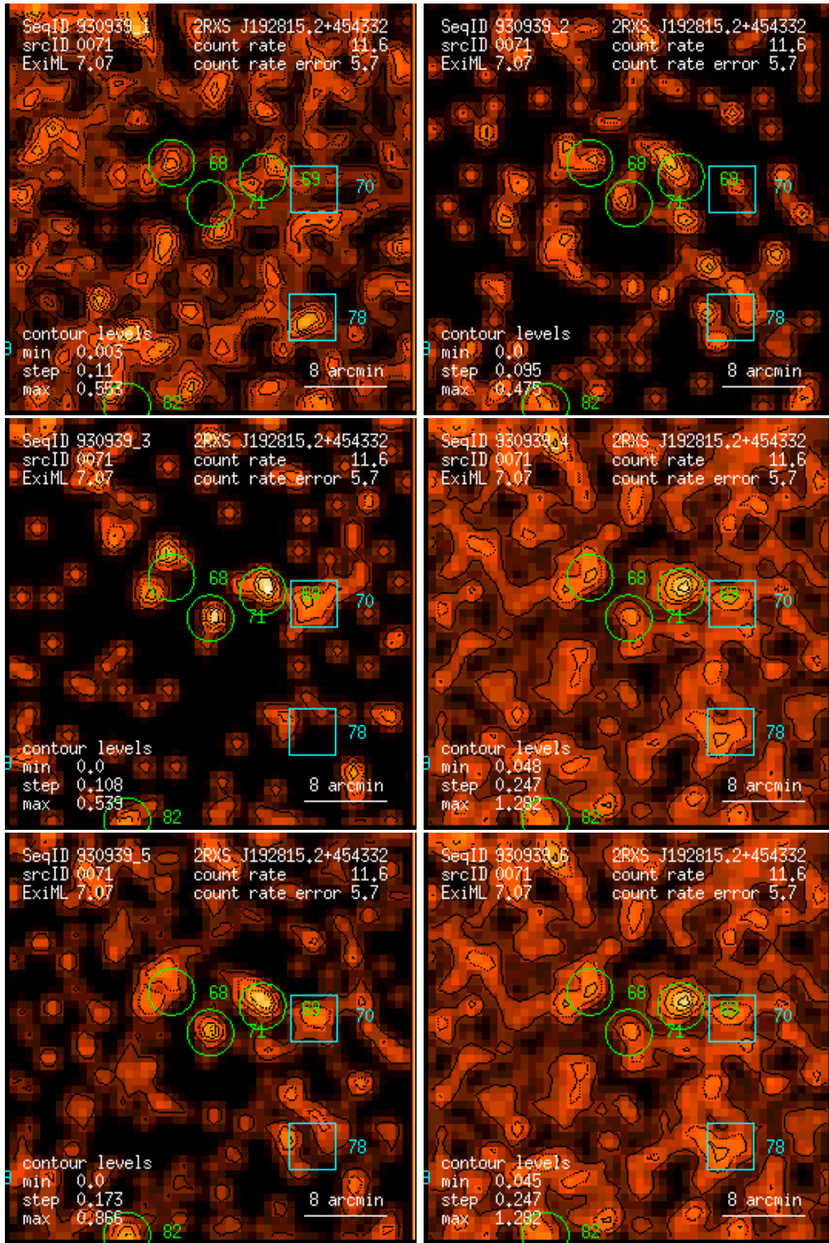
Figure 71: RASS 930939: detection 0071: band rate images, Gaussian filter: (1) PSPC channels 11 – 41, (2) 52 – 90, (3) 91 – 201, (4) 11 – 235, (5) 52 – 201, (6) 11 – 201. Broad band rates in counts/ks. Band rate contour levels in counts/ks/arcmin 2 .
