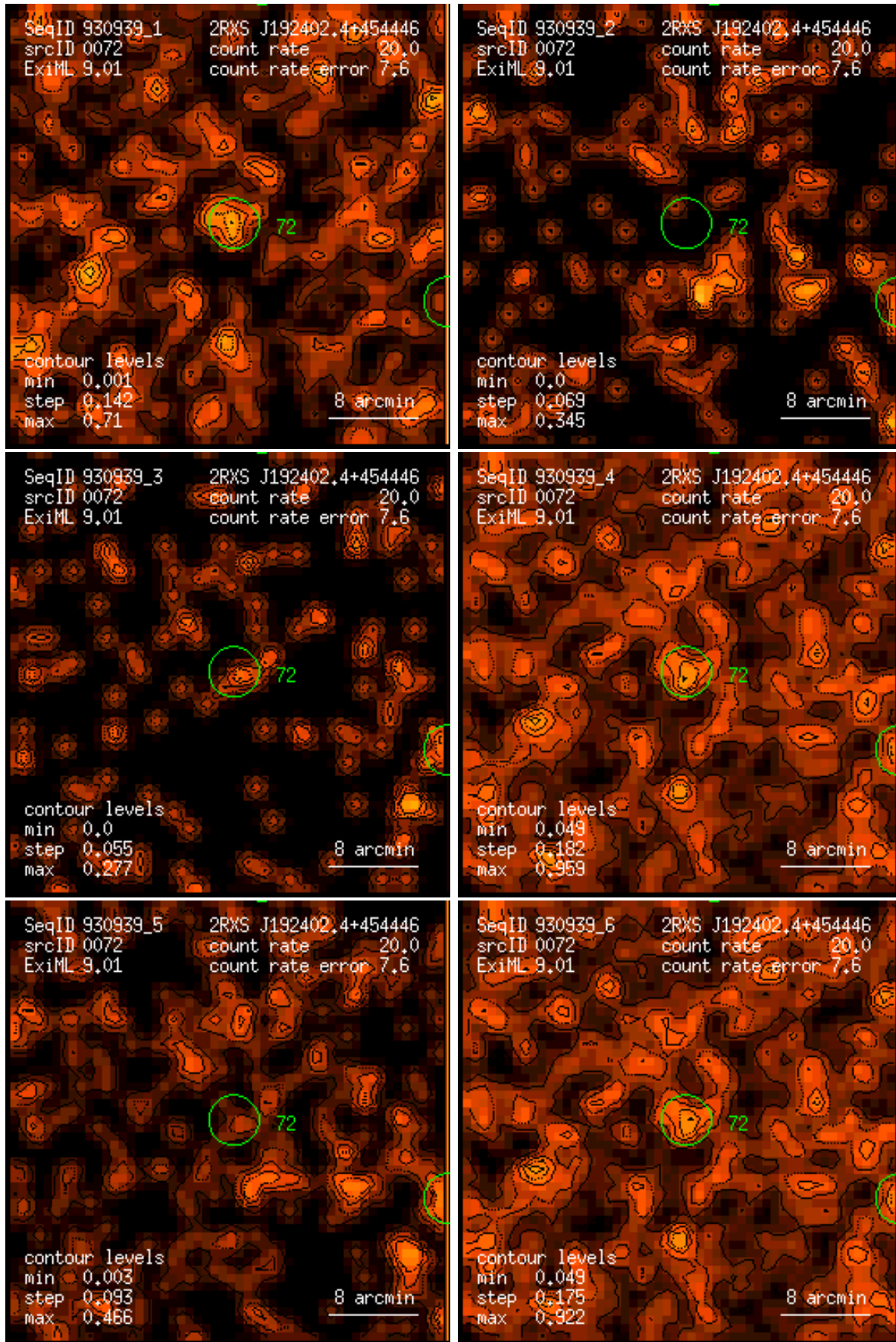
Figure 72: RASS 930939: detection 0072: band rate images, Gaussian filter: (1) PSPC channels 11 – 41, (2) 52 – 90, (3) 91 – 201, (4) 11 – 235, (5) 52 – 201, (6) 11 – 201. Broad band rates in counts/ks. Band rate contour levels in counts/ks/arcmin 2 .
