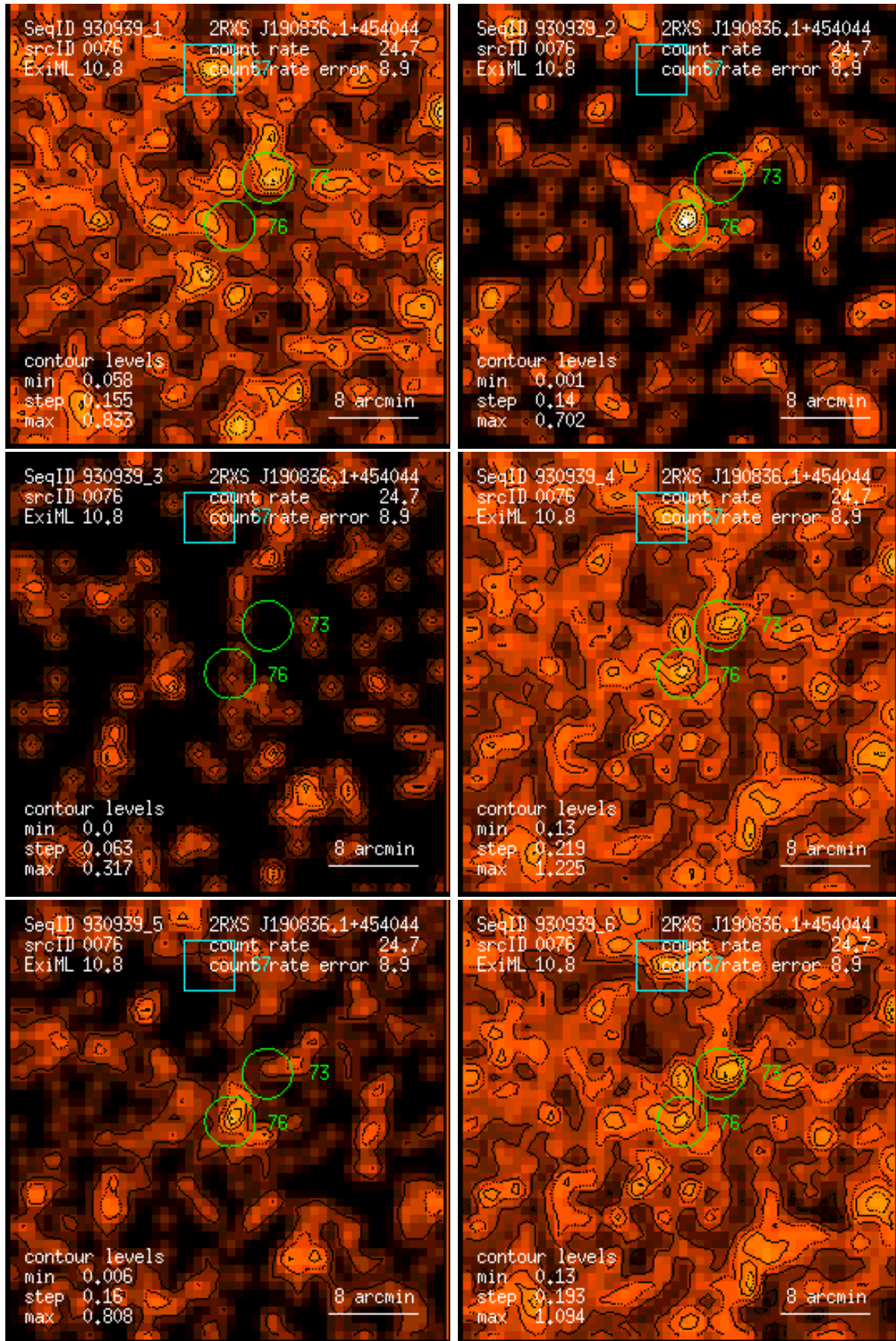
Figure 76: RASS 930939: detection 0076: band rate images, Gaussian filter: (1) PSPC channels 11 – 41, (2) 52 – 90, (3) 91 – 201, (4) 11 – 235, (5) 52 – 201, (6) 11 – 201. Broad band rates in counts/ks. Band rate contour levels in counts/ks/arcmin 2 .
