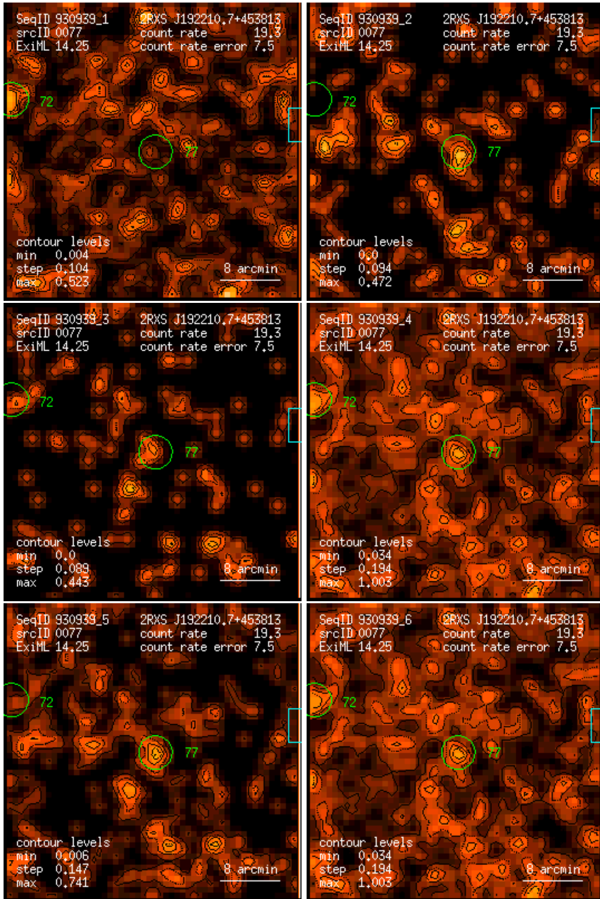
Figure 77: RASS 930939: detection 0077: band rate images, Gaussian filter: (1) PSPC channels 11 – 41, (2) 52 – 90, (3) 91 – 201, (4) 11 – 235, (5) 52 – 201, (6) 11 – 201. Broad band rates in counts/ks. Band rate contour levels in counts/ks/arcmin 2 .
