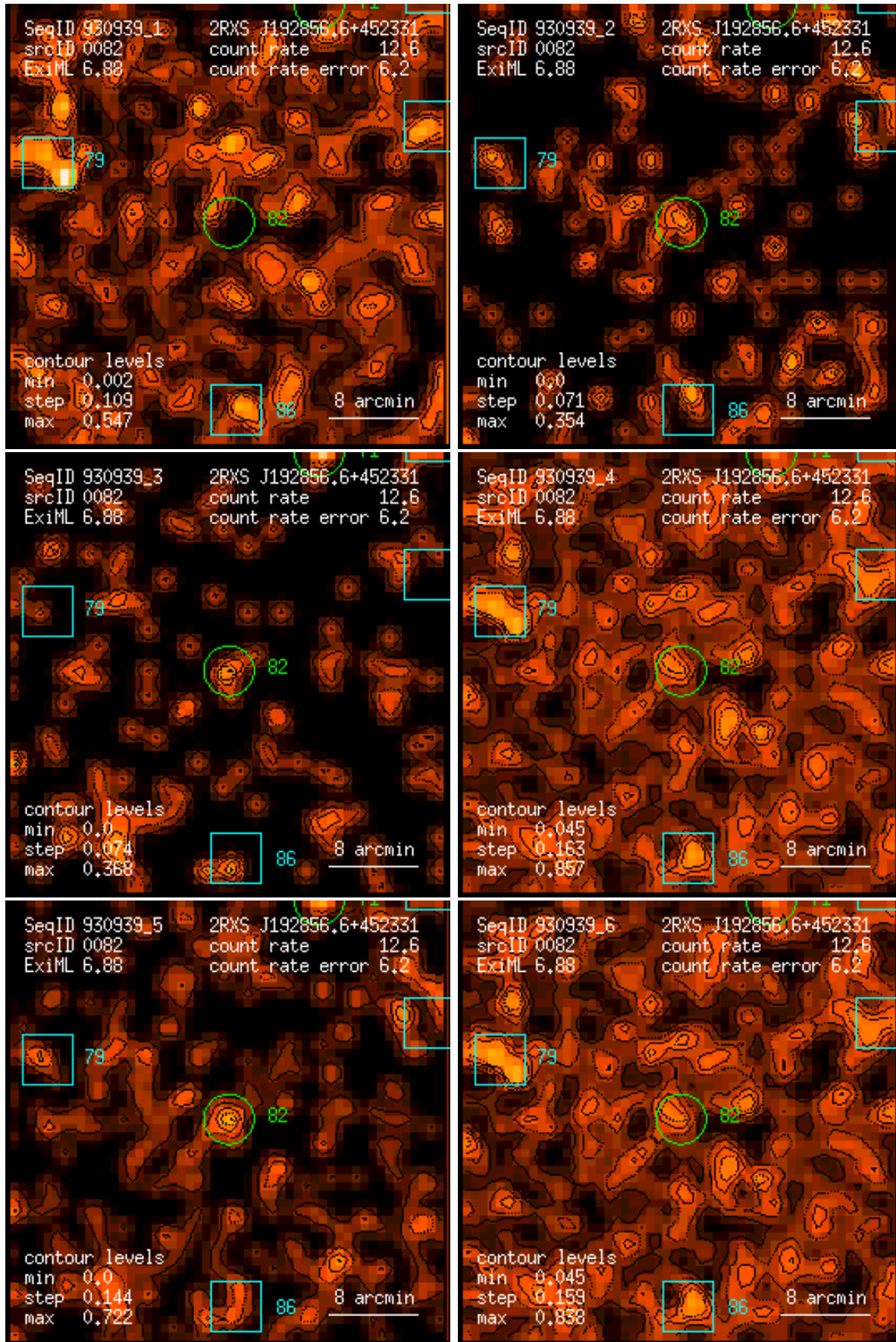
Figure 82: RASS 930939: detection 0082: band rate images, Gaussian filter: (1) PSPC channels 11 – 41, (2) 52 – 90, (3) 91 – 201, (4) 11 – 235, (5) 52 – 201, (6) 11 – 201. Broad band rates in counts/ks. Band rate contour levels in counts/ks/arcmin 2 .
