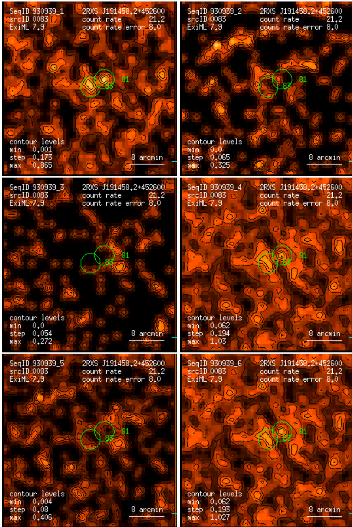
Figure 83: RASS 930939: detection 0083: band rate images, Gaussian filter: (1) PSPC channels 11 – 41, (2) 52 – 90, (3) 91 – 201, (4) 11 – 235, (5) 52 – 201, (6) 11 – 201. Broad band rates in counts/ks. Band rate contour levels in counts/ks/arcmin 2 .
