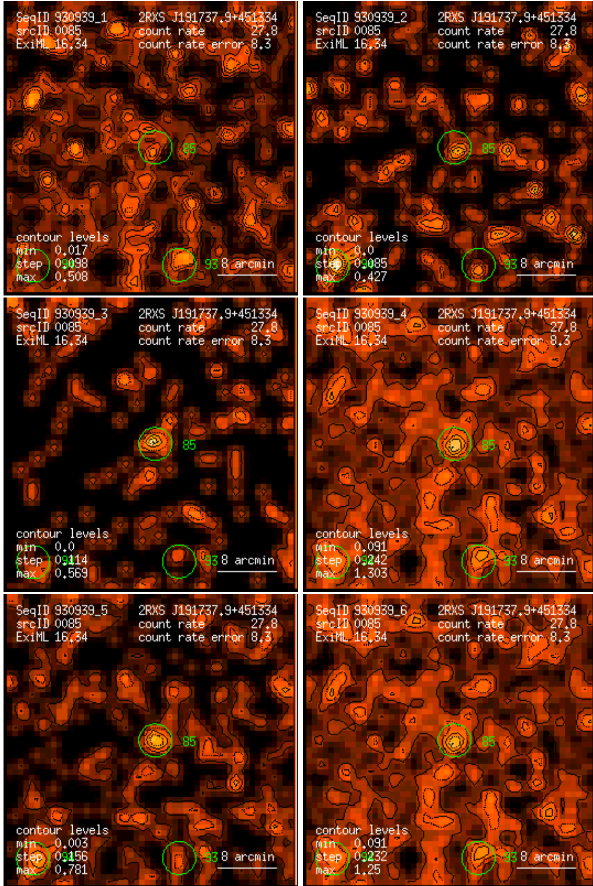
Figure 85: RASS 930939: detection 0085: band rate images, Gaussian filter: (1) PSPC channels 11 – 41, (2) 52 – 90, (3) 91 – 201, (4) 11 – 235, (5) 52 – 201, (6) 11 – 201. Broad band rates in counts/ks. Band rate contour levels in counts/ks/arcmin 2 .
