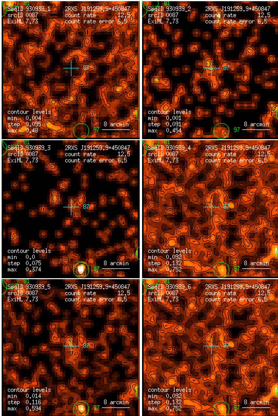
Figure 87: RASS 930939: detection 0087: band rate images, Gaussian filter: (1) PSPC channels 11 – 41, (2) 52 – 90, (3) 91 – 201, (4) 11 – 235, (5) 52 – 201, (6) 11 – 201. Broad band rates in counts/ks. Band rate contour levels in counts/ks/arcmin 2 .
