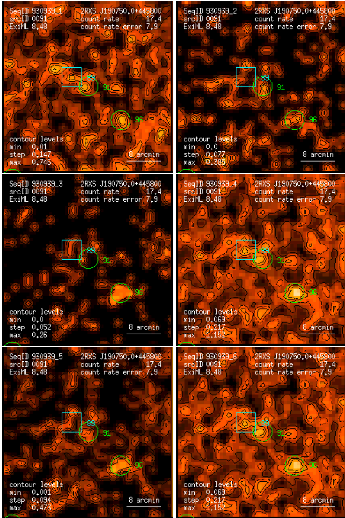
Figure 91: RASS 930939: detection 0091: band rate images, Gaussian filter: (1) PSPC channels 11 – 41, (2) 52 – 90, (3) 91 – 201, (4) 11 – 235, (5) 52 – 201, (6) 11 – 201. Broad band rates in counts/ks. Band rate contour levels in counts/ks/arcmin 2 .
