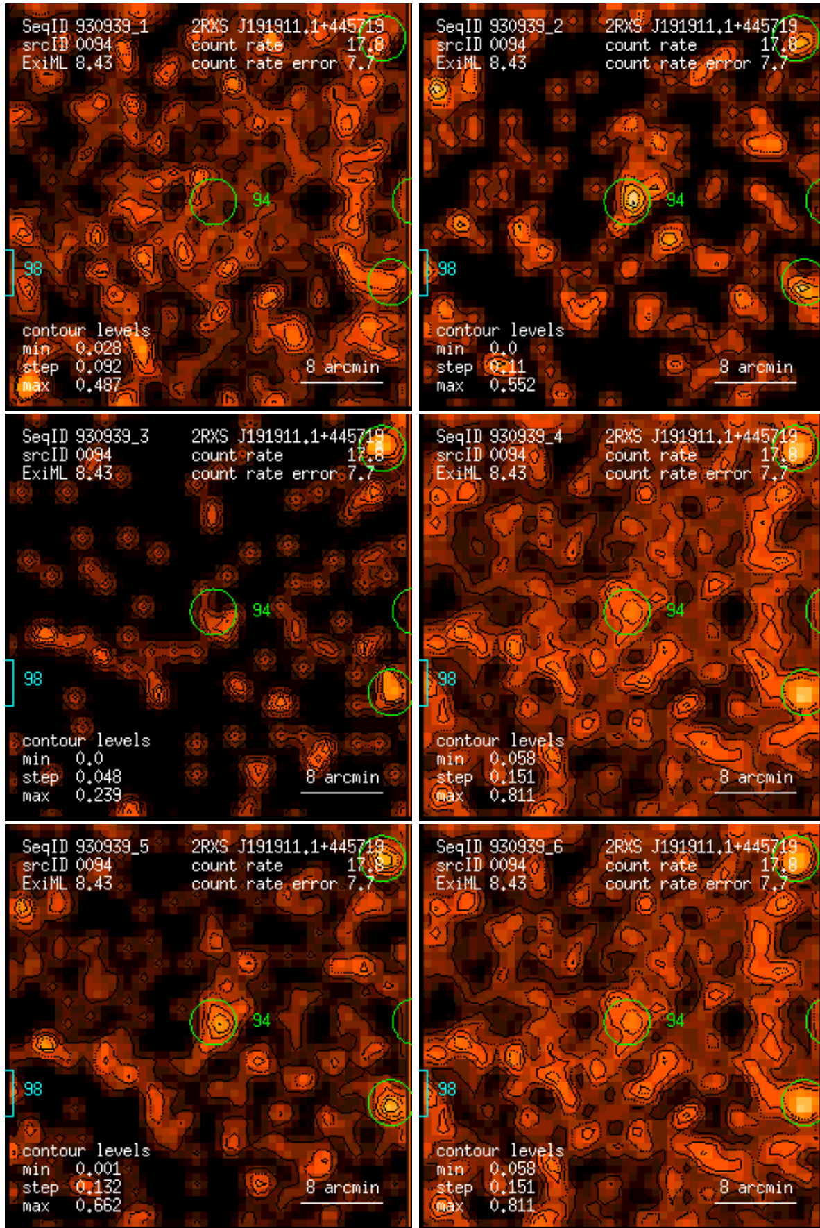
Figure 94: RASS 930939: detection 0094: band rate images, Gaussian filter: (1) PSPC channels 11 – 41, (2) 52 – 90, (3) 91 – 201, (4) 11 – 235, (5) 52 – 201, (6) 11 – 201. Broad band rates in counts/ks. Band rate contour levels in counts/ks/arcmin 2 .
